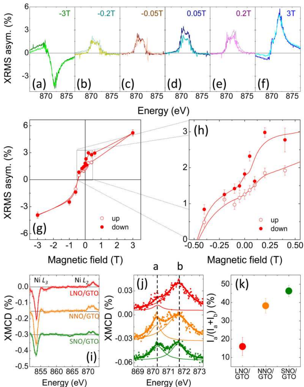
FIGURE 6. Role of covalence on magnetism
