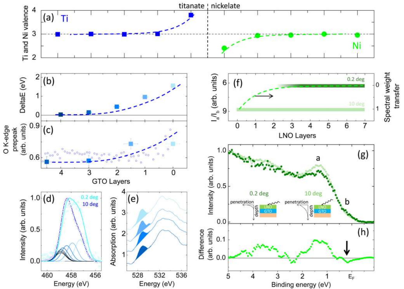
FIGURE 2. Interfacial charge transfer in \text{LaNiO}_3/\text{GdTiO}_3
