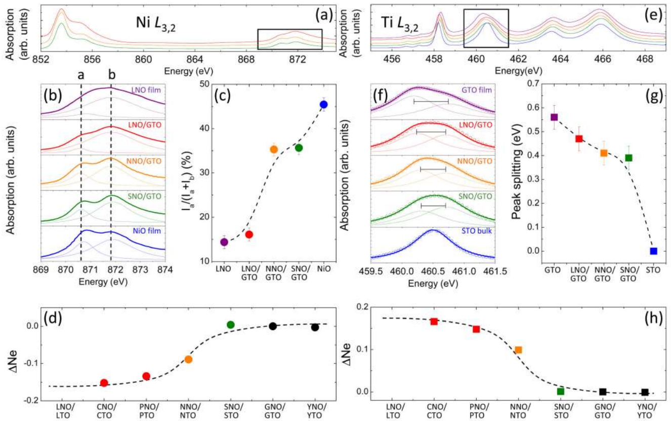
FIGURE 3. Tuning interfacial charge transfer by the rare earth in the nickelate
