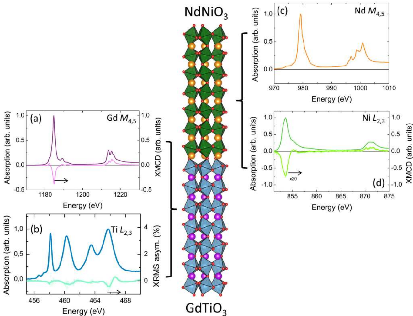
FIGURE 5. Induced magnetic moment in the nickelates
