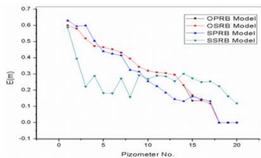
Fig. 5. Specific energy graphical representation for 6m head
