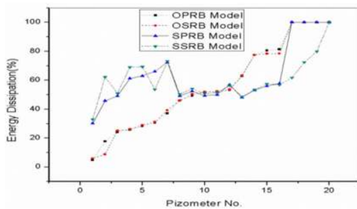
Fig. 6. Energy dissipation for ogee and stepped spillway at low head
