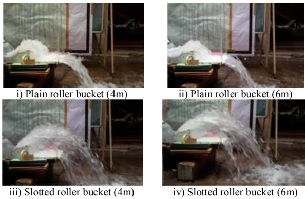
Fig. 3. Hydraulic jump on roller buckets without stilling basin
