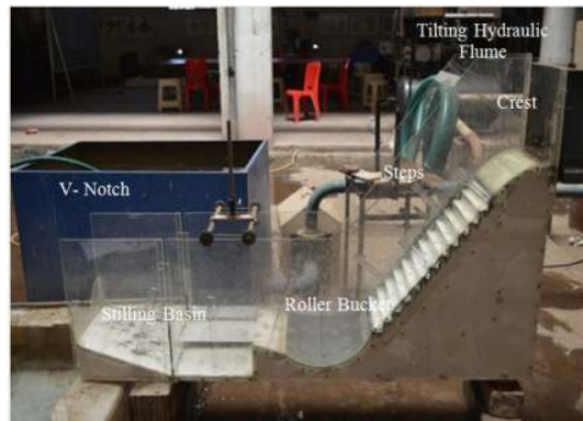
Fig. 2. Hydraulic model of the ogee profile stepped spillway
