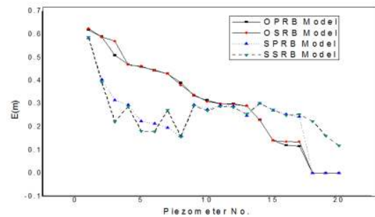
Fig. 4. Specific energy for ogee and stepped spillway model at low head
