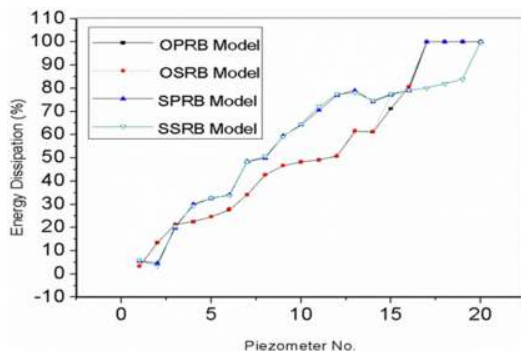
Fig. 7. Energy dissipation for ogee and stepped spillway at high head
