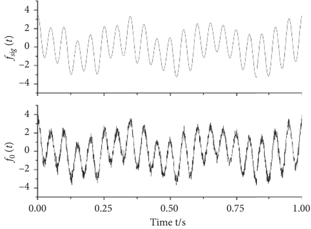
FIGURE 2: Time-domain diagram of f_{\text{sig}}(t) signal and f_o(t) signal.
