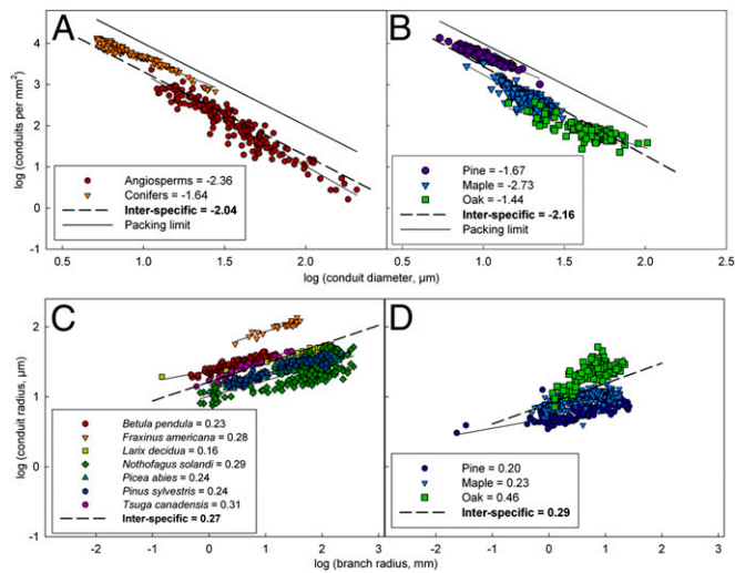
Fig. 3. Plots of the packing rule and the conduit taper. For the packing rule A is reproduced from ref. 2, and B shows our measurements. For the taper C shows literature data ( SI Text ; Table S2 ) and D shows our measurements. Each colored symbol represents a different species. The packing limits in both plots (upper lines) represent wood tissue composed entirely of closest-packed conduits (i.e., the closest packing of both square-shaped conduits in conifers and circular-shaped conduits in angiosperms).
