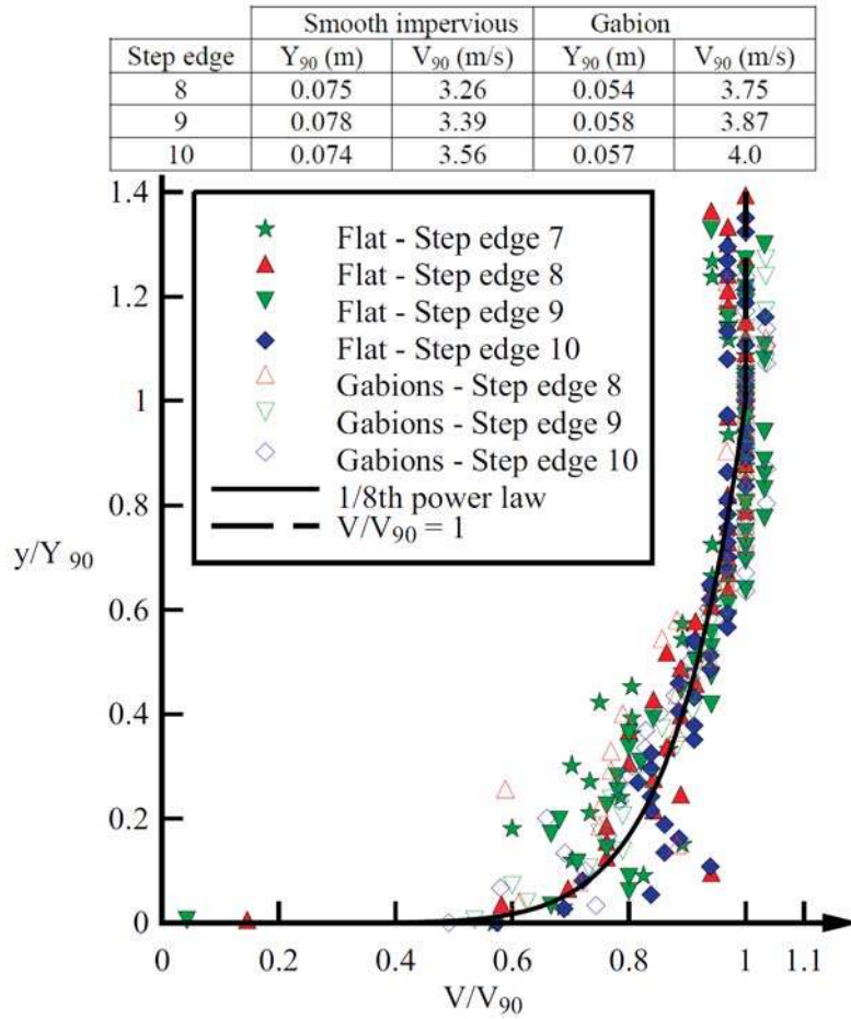
Fig. 6 - Velocity distributions in skimming flow on smooth impervious and gabion stepped weirs - \theta = 26.6^\circ , h = 0.10 m, d_c/h = 1.3 , Q = 0.076 m 3 /s, Re = 5.9 \times 10^5 - Comparison with a 1/8th profile
