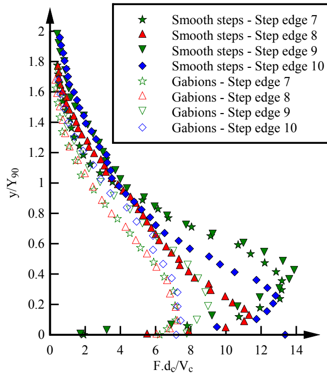
Fig. 5 - Bubble count rate distributions in transition and skimming flows on smooth impervious and gabion stepped weirs - \theta = 26.6^\circ , h = 0.10 m (A) d_c/h = 0.5 , Q = 0.018 m 3 /s, Re = 1.40 \times 10^5
