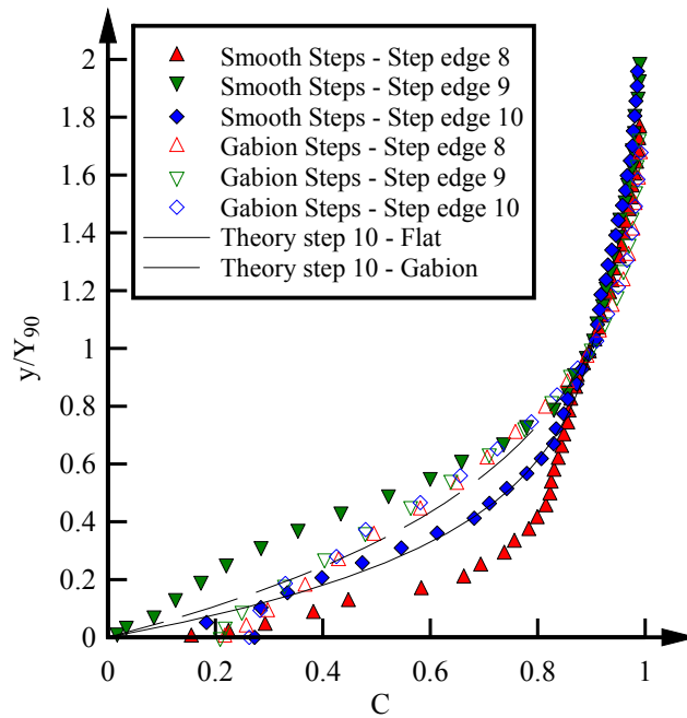
Fig. 4 - Air concentration distributions in transition and skimming flows on smooth impervious and gabion stepped weirs - \theta = 26.6^\circ , h = 0.10 m
