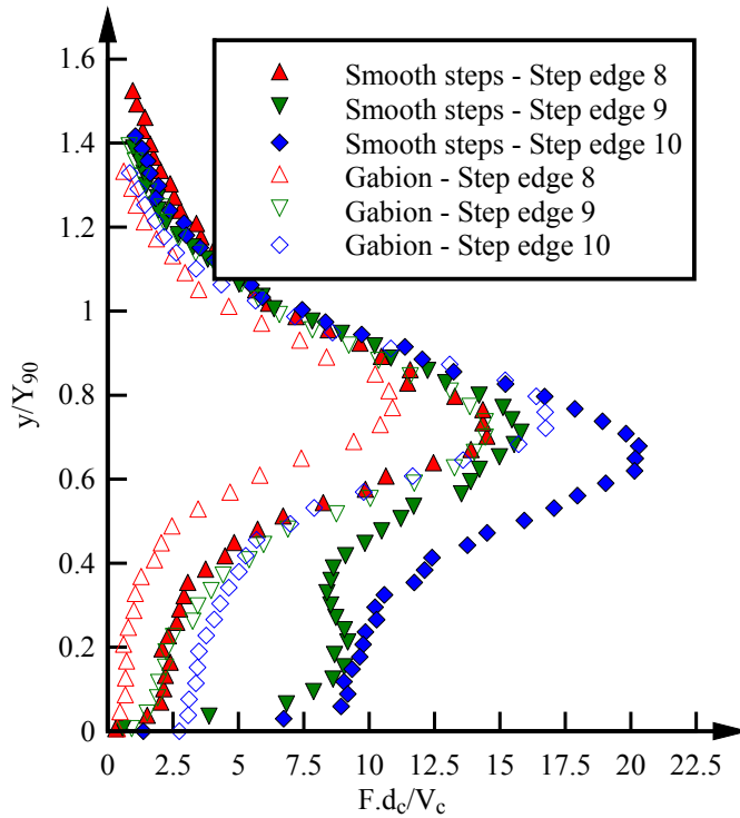
(B) d_c/h = 1.5 , Q = 0.095 m 3 /s, Re = 7.3 \times 10^5
