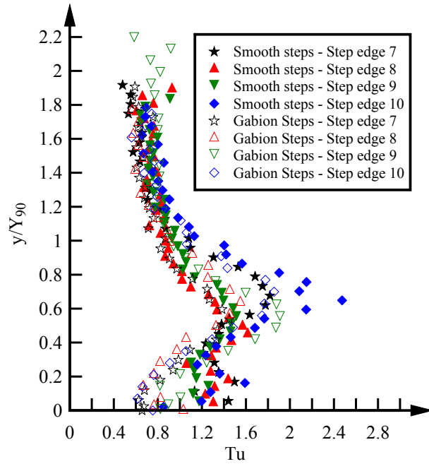
Fig. 7 - Turbulence intensity distributions in transition and skimming flow in smooth impervious and gabion stepped weirs - \theta = 26.6^\circ , h = 0.10 m
