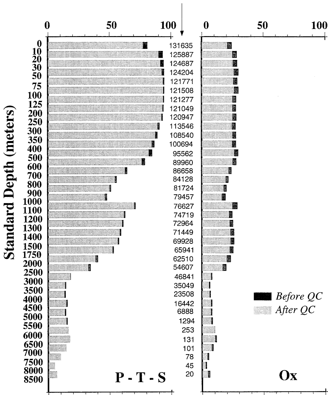
Figure 2: Vertical distribution of observations in North Atlantic dataset from Lozier et al. (1996) (only stations > 200 meters are included here) before and after quality control procedures. Each bar depicts the percentage of stations in which at least one observation was made between the standard depths listed on the y-axis. This percentage is based only on the number of stations where the sea floor is deeper than the standard depth.
