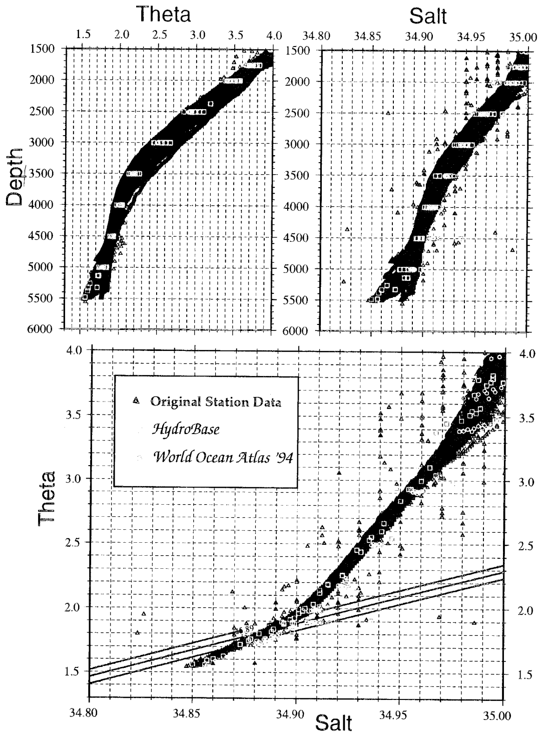
Figure 7: Potential temperature and salinity from a 5^\circ square geographical area near 25^\circ\text{N} , 72^\circ\text{W} plotted vs. depth and in \theta -S space compares averaged values from HydroBase and World Ocean Atlas 1994 (Levitus, 1994) to the original observations from which both were derived. Selected density contours (45.89, 45.90, and 45.91) are also mapped onto the \theta -S diagram. The WOA salinities are significantly higher than the observations near 4500 meters leading to a skewed \theta -S curve. The WOA omits nearly all data > 5000 because most stations do not reach to the next standard depth level, 5500m. The result is that the deepest part of the \theta -S curve is not represented at all in the WOA dataset.
