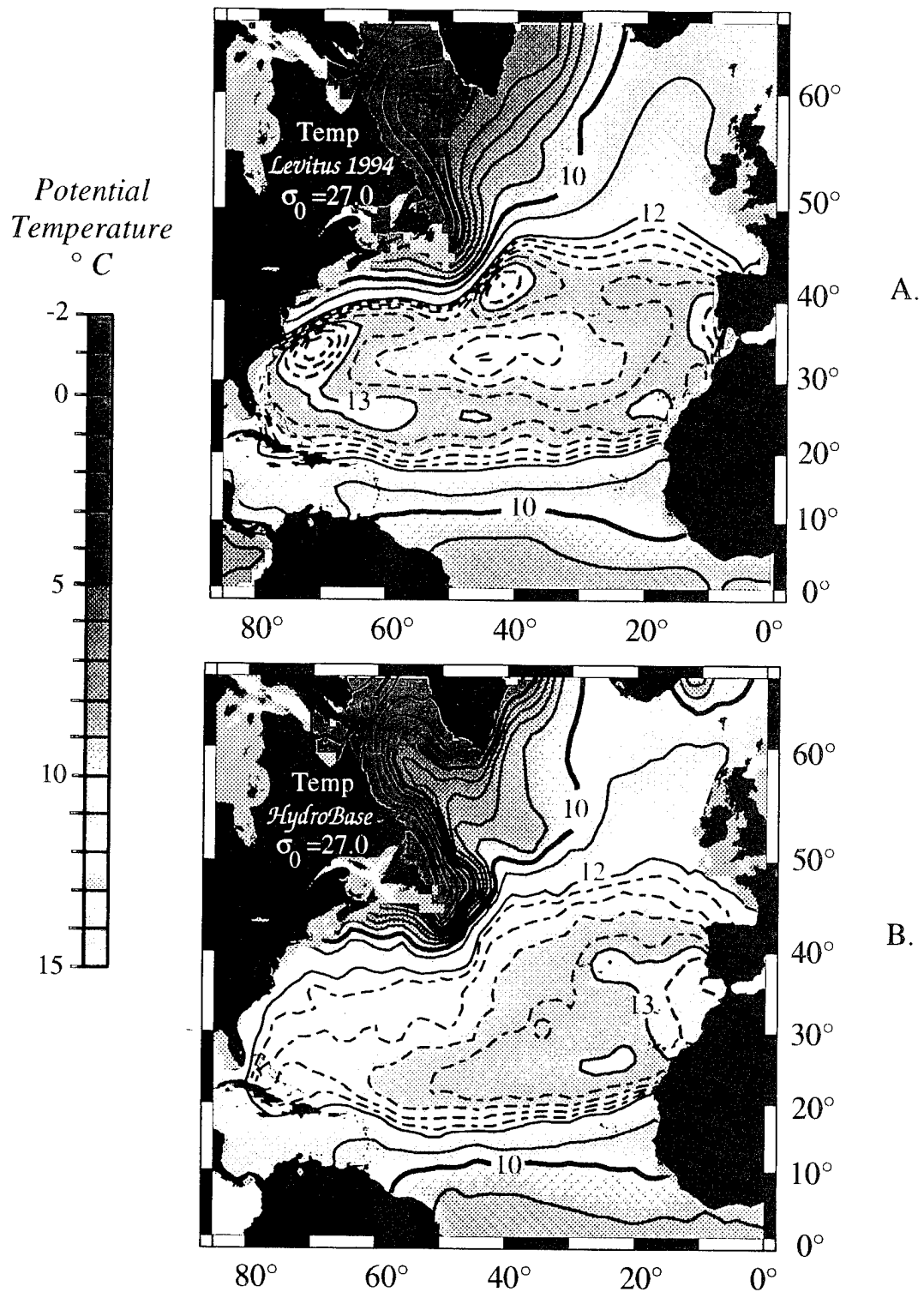
Figure 3: Potential temperature on a density surface in the thermocline of the subtropical gyre from A) Levitus' World Ocean Atlas 1994 database and B) HydroBase . Both represent the 1° gridded annual averages which were treated identically to produce these maps. The WOA map contains anomalously warm (red) patches along 28°N and in the Gulf Stream system, and anomalously cooler temperatures (closed yellow contours) in the center of the subtropical gyre. Isopycnal averaging is one factor in avoiding such anomalies.
