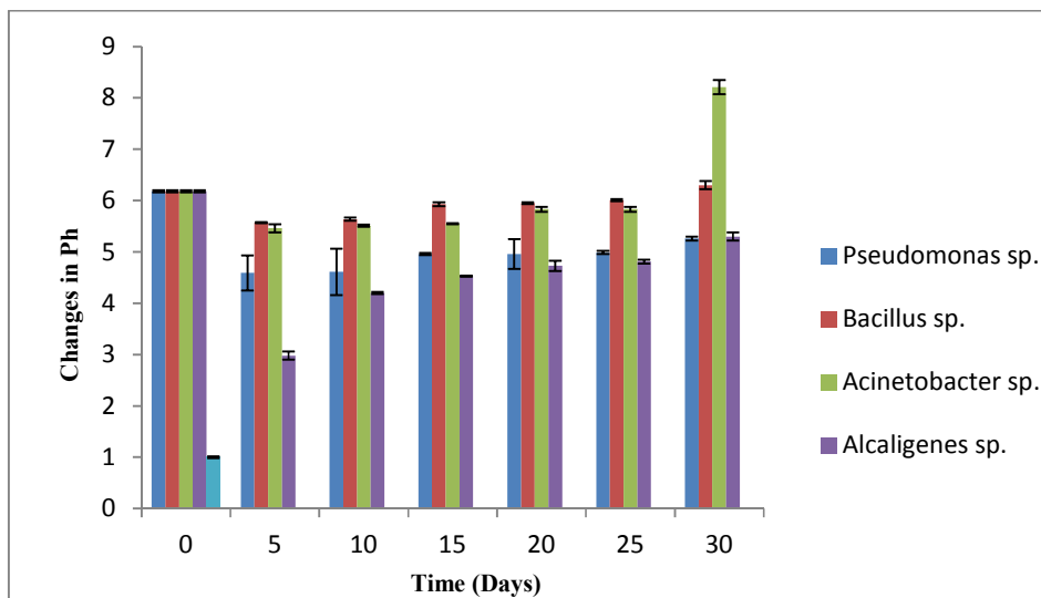
Fig. 5. Changes in pH against time in (Days) caused by some of the isolates during the degradation studies (Data are mean ±S.D of triplicate determinations)
