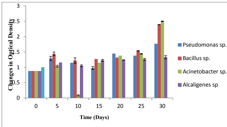
Fig. 3. Changes in optical density (OD) against time in (Days)caused by some of the isolates during the degradation studies (Data are mean \pm S.D of triplicate determinations)
