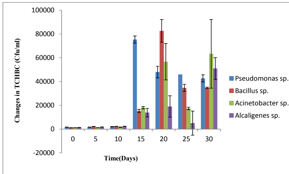
Fig. 6. Changes in total cuturable heterotrophic bacteria counts (cfu/ml) against Time in (Days) caused by some of the isolates during the degradation studies (Data are mean \pm S.D of triplicate determinations)
