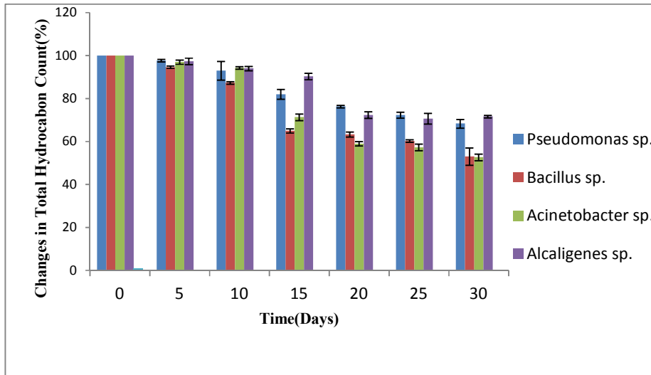
Fig. 2. Changes in total hydrocarbon content (%) against time(Days)caused by some of the isolates during the degradation studies (Data are mean \pm S.D of triplicate determinations)
