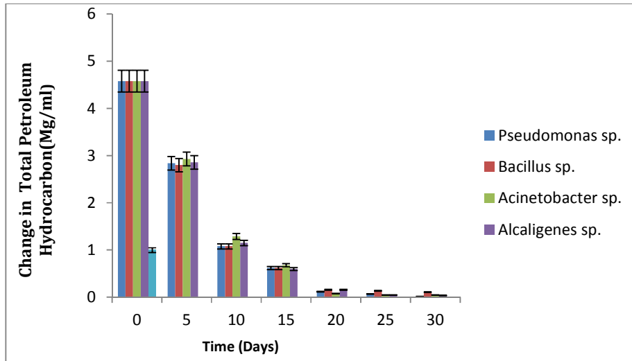
Fig. 4. Changes in total petroleum hydrocarbon in (mg/ml) against time in (Days) caused by some of the isolates during the degradation studies (Data are mean ±S.D of triplicate determinations)
