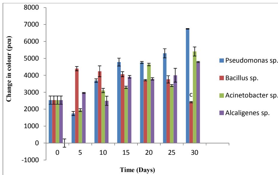
Fig. 1. Changes in colour (pcu) against time(days) caused by some of the isolates during the degradation studies (data are mean \pm s.d of triplicate determinations)
