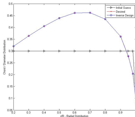
Figure 4 Results of propeller inverse design
