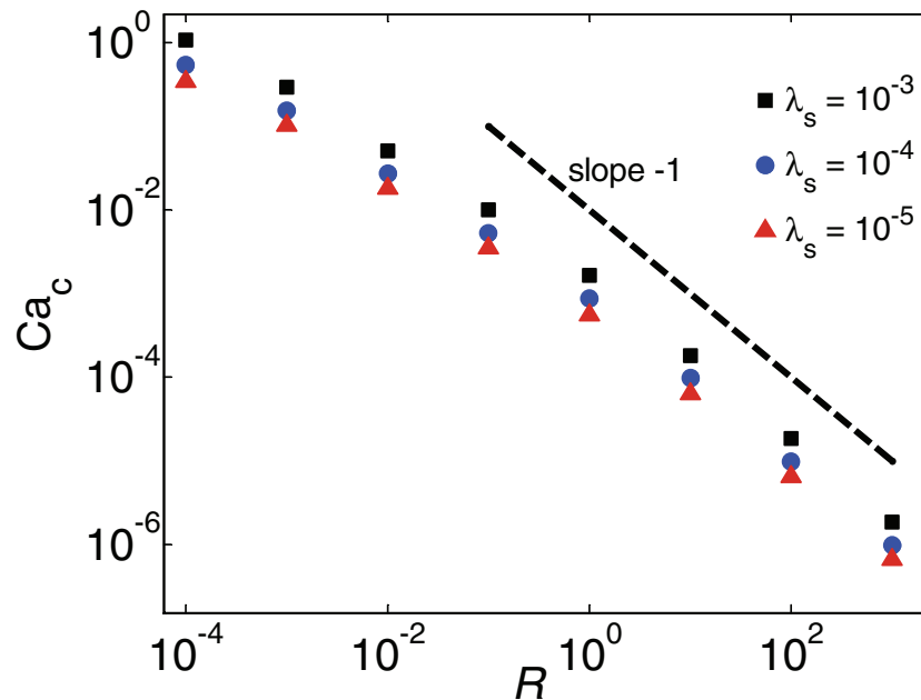
FIG. 9. Critical capillary number Ca_c versus viscosity ratio R for different slip lengths \lambda_s ( \theta_e = 2.8 rad). The dashed line indicates a power law with exponent -1 , which is valid for large R .
