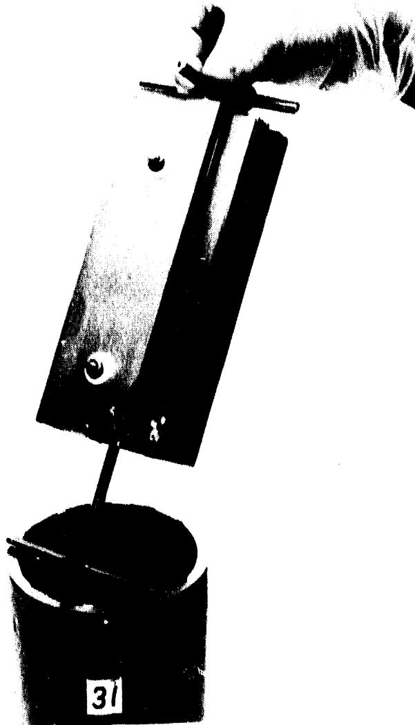
Figure 6-7. Post-test appearance of steel specimens, vapor-phase exposure, 24-month brine/CO 2 tests. No significant corrosion reaction is evident except where brine has contacted the bottoms of the specimens.
