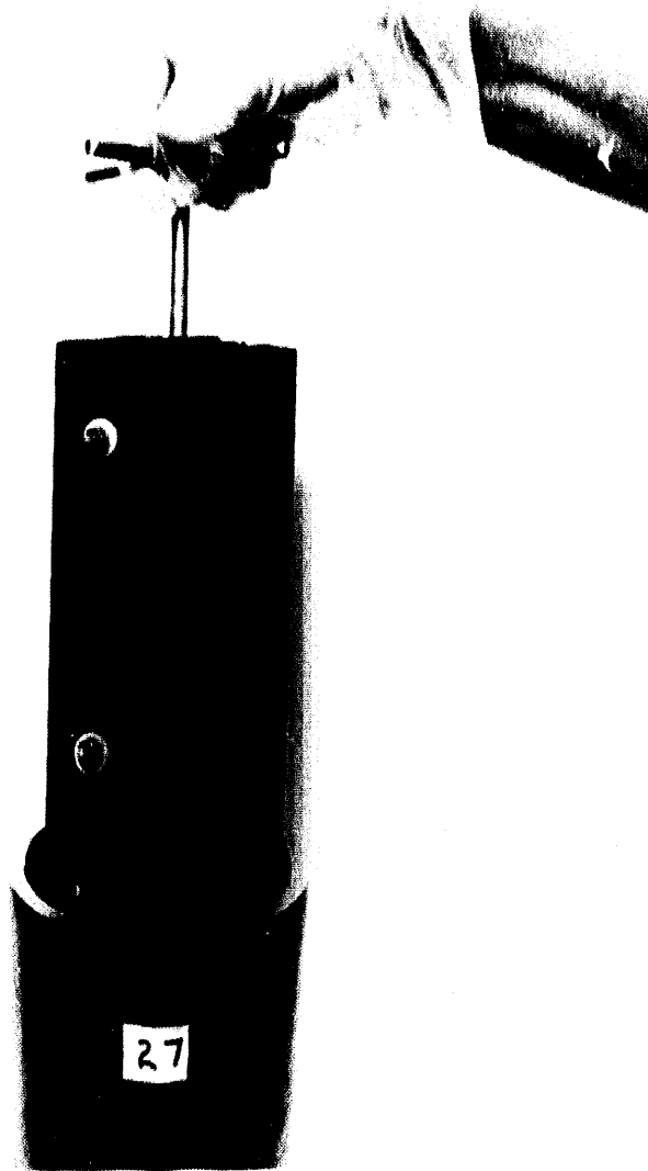
Figure 6-6. Post-test appearance of steel specimens, immersed, 24-month brine/ \text{CO}_2 tests. Specimens are coated with an adherent black \text{FeCO}_3 corrosion product.
