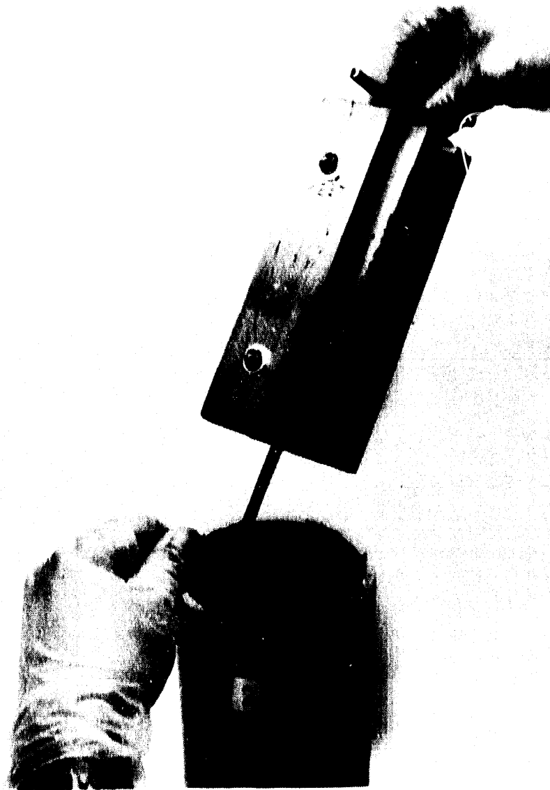
Figure 6-3. Post-test appearance of steel specimens, vapor-phase exposure, 24-month anoxic brine tests. No reaction is evident except where brine has contacted the bottoms of the specimens.
