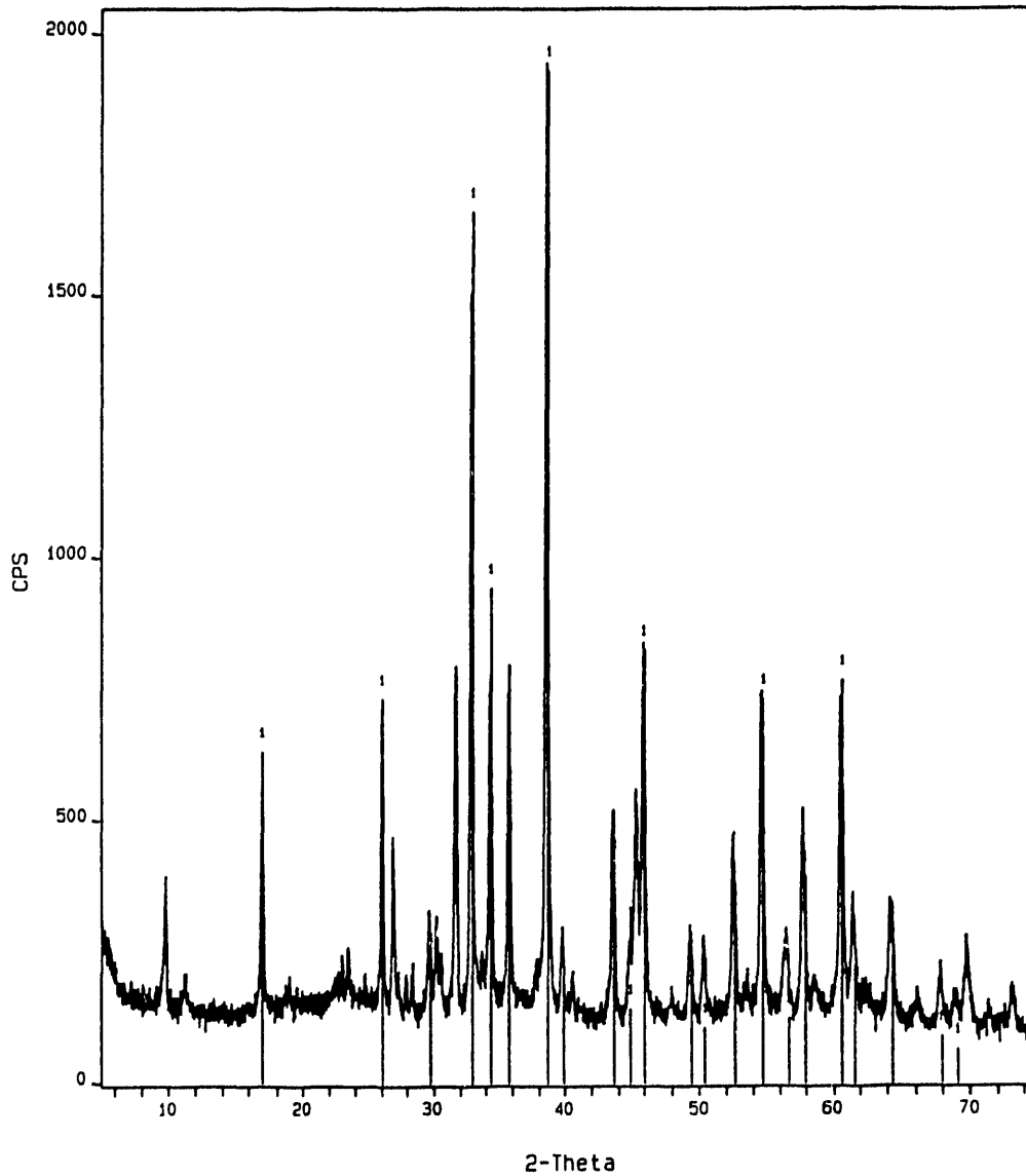
Figure 6-4. XRD results obtained from the unidentifiable 12- and 24-month-test corrosion products, anoxic brine tests. The vertical lines (labeled "1") correspond to the principal 12-month corrosion-product diffraction peaks; they are superimposed on the raw data obtained from the 24-month corrosion product. More than one compound may be present in each lot of corrosion product.
