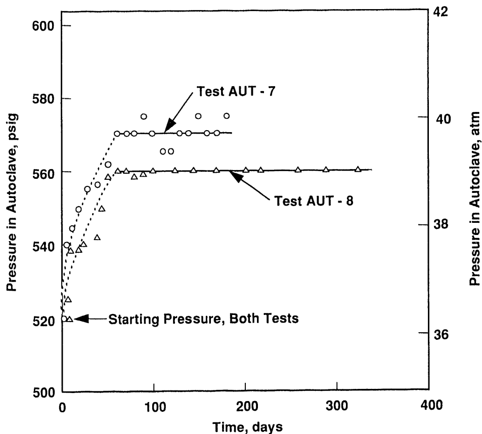
Figure 6-10. Pressure-time curves, tests AUT-7 and AUT-8.
