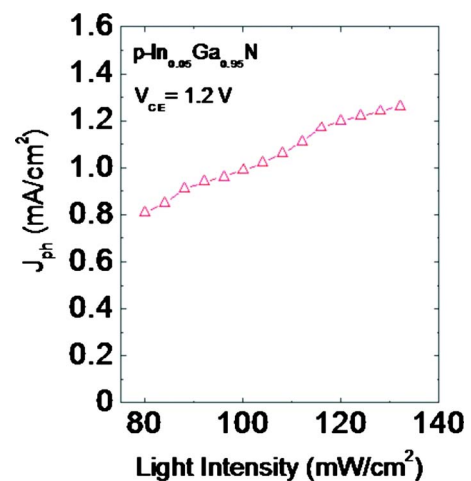
FIG. 4. (Color online) Photocurrent densities ( J_{ph} ) of p-In 0.05 Ga 0.95 N as a function of light intensity at V_{CE} =1.2 V.
