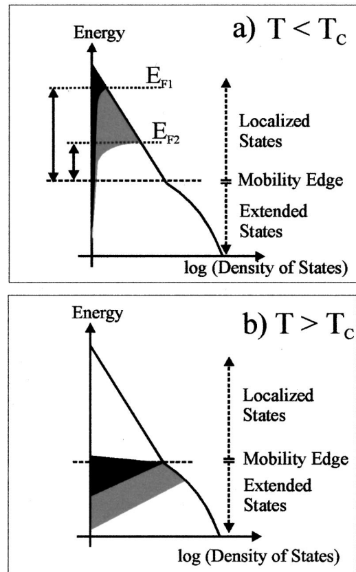
FIG. 3. Exponential tail of localized states at the valence band edge. At temperature below T_c holes are localized in the tail. Only a small fraction can propagate in extended states (a). Above T_c most of the holes are thermally excited into extended states of the valence band (b). The black and gray regions represent two hole densities. E_{F1} and E_{F2} are the activation energies of trapped holes.
