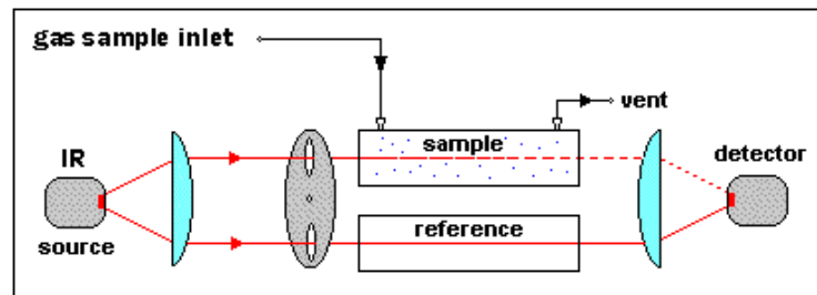
Figure 3.4: Schematic representation of the NDIR principle [113].
