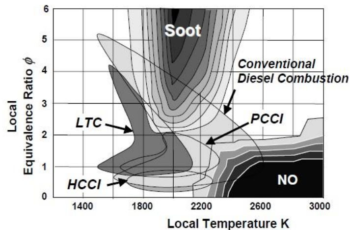
Figure 2.9: Equivalence ratio-temperature diagram of different combustion concepts [48].
