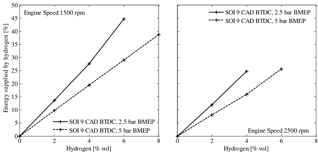
Figure 4.2: Diagram of the energy supplied by hydrogen.
