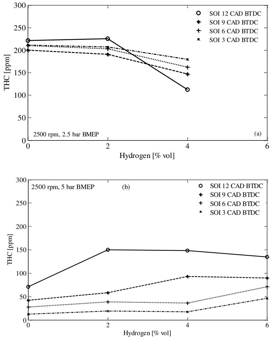
Figure 4.9: Effect of intake air enrichment with hydrogen on the unburned hydrocarbons. Engine speed: 2500 rpm, load: (a) 2.5 bar BMEP, (b) 5 bar BMEP.
