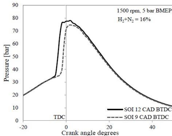
Figure 6.7: Comparison of the in-cylinder pressure data. Engine speed: 1500 rpm, load: 5 bar BMEP, SOI: 12 and 9 CAD BTDC, H_2 + N_2 vol. fraction 16%.
