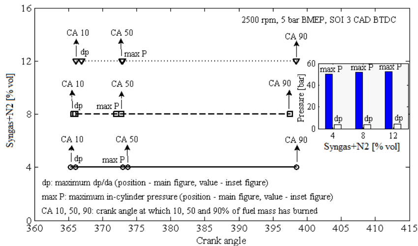
Figure 7.12: Mass fraction burned, maximum pressure rise rate and maximum pressure Engine speed 2500 rpm, load 5 bar BMEP, SOI 3 CAD BTDC.
