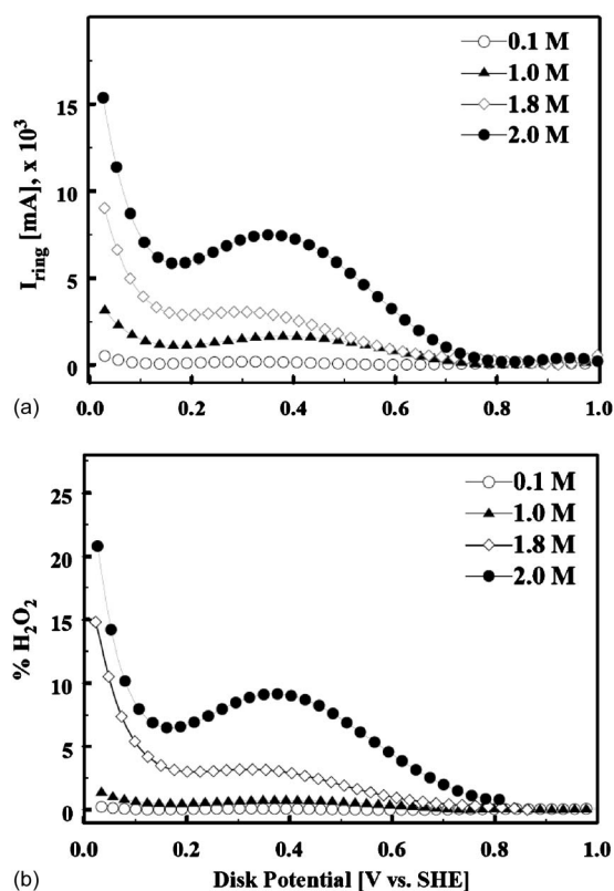
Figure 4. (a) Rate and (b) % of H 2 O 2 formed during the oxygen reduction reaction on Pt/Vulcan XC-72R in 0.1 M [○], 1.0 M [▲], 1.8 M [◇] and 2.0 M [●] HClO 4 solution [pH - 0.3] bubbled with O 2 at 25°C. E_{ring} = 1.2 V vs SHE, 1 mV/s, 2500 rpm.
