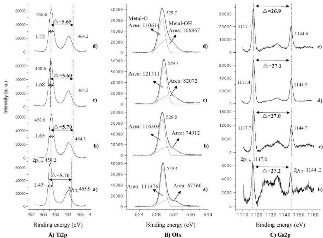
Figure 5. XPS of \text{TiO}_2 and Ga- \text{TiO}_2 as-synthesized: (A) For Ti2p, (B) For O1s, and (C) For Ga2p: (a) pure \text{TiO}_2 , (b) 1.0 mol% Ga- \text{TiO}_2 , (c) 2.0 mol% Ga- \text{TiO}_2 , and (d) 5.0 mol% Ga- \text{TiO}_2 .
