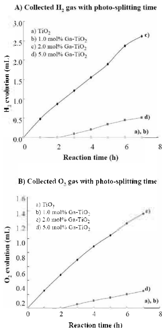
Figure 6. The H 2 evolution from water photo splitting over pure TiO 2 and Ga-TiO 2 : (a) pure TiO 2 , (b) 1.0 mol% Ga-TiO 2 , (c) 2.0 mol% Ga-TiO 2 , and (d) 5.0 mol% Ga-TiO 2 .
