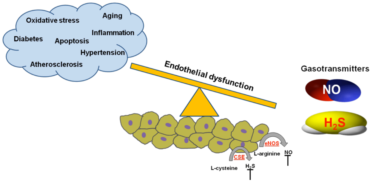
Figure 2. H 2 S and NO maintain different EC functions
