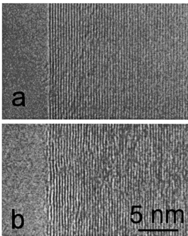
Figure 6. TEM images of pristine (a) and hydrogenated (b) graphite flakes.
