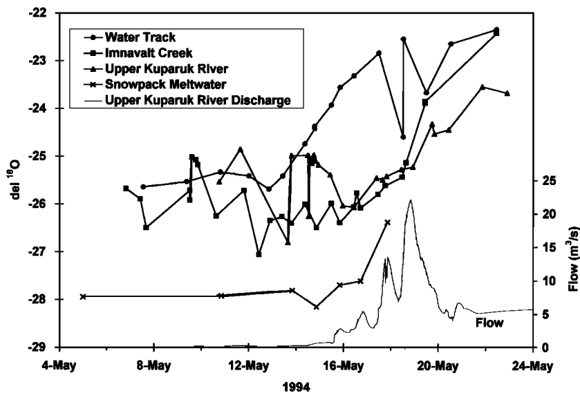
Figure 6. The ^{18}\text{O} contents for the Upper Kuparuk River, Imnavait Creek, the hillslope water track, and snowpack meltwater during the 1994 snowmelt period. The snowmelt hydrograph for the Upper Kuparuk River is shown for reference.
