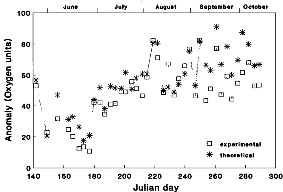
Fig. 9. Evolution in time of theoretical ( 175 [\text{HPO}_4^{2-}]^s ) and experimental ( [\text{O}_2]^s ) oxygen consumption due to remineralization processes over the shelf at 70 m depth.
