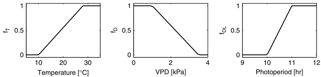
Figure 1. Stress functions for the three environmental variables used in the k_{\text{rubber}} to protect rubber phenology, temperature, vapor pressure deficit and photoperiod or daylength.
