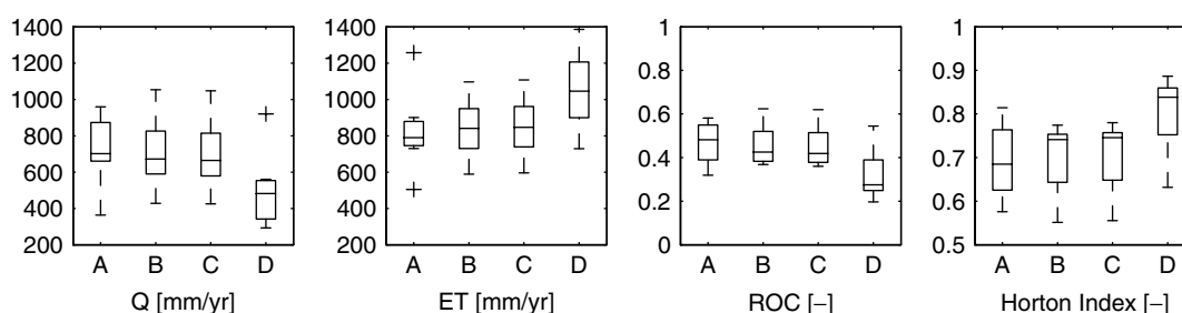
Figure 5. Box plots summarizing the overall water balance. Q is total discharge, ET is total evapotranspiration, and ROC is runoff coefficient. Shown are scenario A: observations; scenario B: baseline simulation; scenario C: rubber simulation using traditional f_{\theta} and f_{\text{LAI}} ; and scenario D: rubber simulation using the proposed crop factor. The top and bottom ends of the box correspond to the 25th and 75th percentiles of the samples, and the centre line is the median. Whiskers extend from each end of the box to the adjacent values in the data and outliers are data with values beyond the ends of the whiskers, displayed with a cross.
