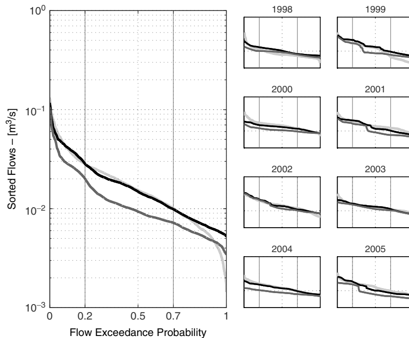
Figure 6. Observed (light grey) and simulated (black) yearly exceedance probability plots for annual and total discharge. Dark grey lines show model results when vegetation is replaced by rubber fields modelled with the K_{\text{rubber}} model (Scenario D).
