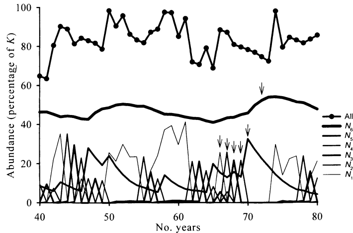
FIG. 3. Example of a projection of the model, using the vital rates in Table 1 and natural flow regime conditions. Abundances are expressed as a percentage of K_T , the total area suitable for cottonwood. Seedlings ( N_1 ) and younger trees ( N_2 – N_5 ) show boom–bust dynamics, while the area covered by mature trees ( N_6 ) fluctuates more moderately. Flood years, where seedling establishment occurs, can be identified by nonzero values for N_1 . Significant recruitment of mature trees occurs when a flood causes high seedling recruitment, and then no floods or droughts occur for several more years (arrows point to an example of this). Self-thinning, flood mortality, and drought mortality leave a substantial amount of suitable cottonwood habitat unoccupied in some years (the total habitat occupied by cottonwood, “All,” is often <100%).
