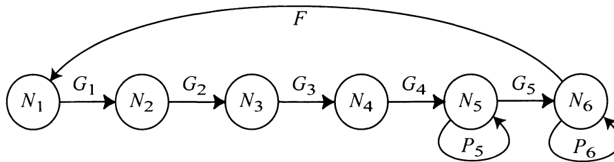
FIG. 1. Life cycle for the cottonwood model. Stage 1 represents seedlings; stages 2–4 are 2–4-yr-olds, respectively; stage 5 represents subadult trees (mostly 5–10-yr-olds); and stage 6 represents reproductive adults. N is abundance, G is the probability of transition to the next stage, P is the probability of remaining in that stage, and F is fecundity.
