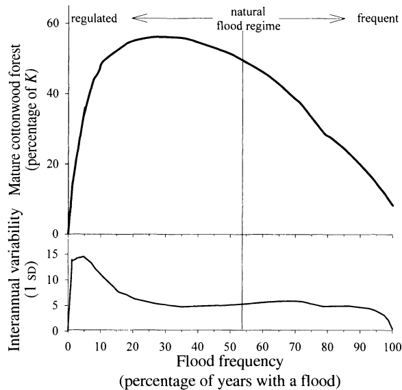
FIG. 4. Effect of altered flood regime on mature cottonwood populations. Flood frequency varies from frequent (a scouring flood every year) to highly regulated (no floods). Top panel: mature cottonwood forest is most abundant when floods are slightly less frequent than the natural flood regime. Bottom panel: interannual variability in coverage is lowest at intermediate and high flood frequencies, while low flood frequencies result in variable populations that sometimes disappear locally from reaches.
