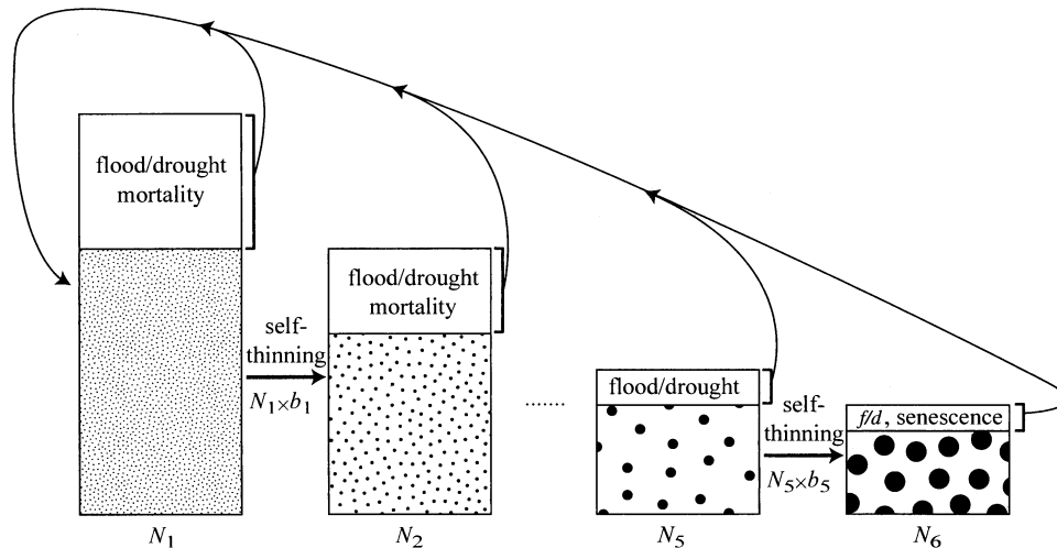
FIG. 2. Schematic showing how stand structure is represented in the cottonwood model. Every year, a fraction of each stand may be lost to flood or drought mortality. This space becomes available for colonization by new seedlings the following year (if conditions favor seedling recruitment). Within the remaining portions of stands, self-thinning occurs at rate b so that the number of individuals in a stand decreases while the space occupied by a stand remains constant.
