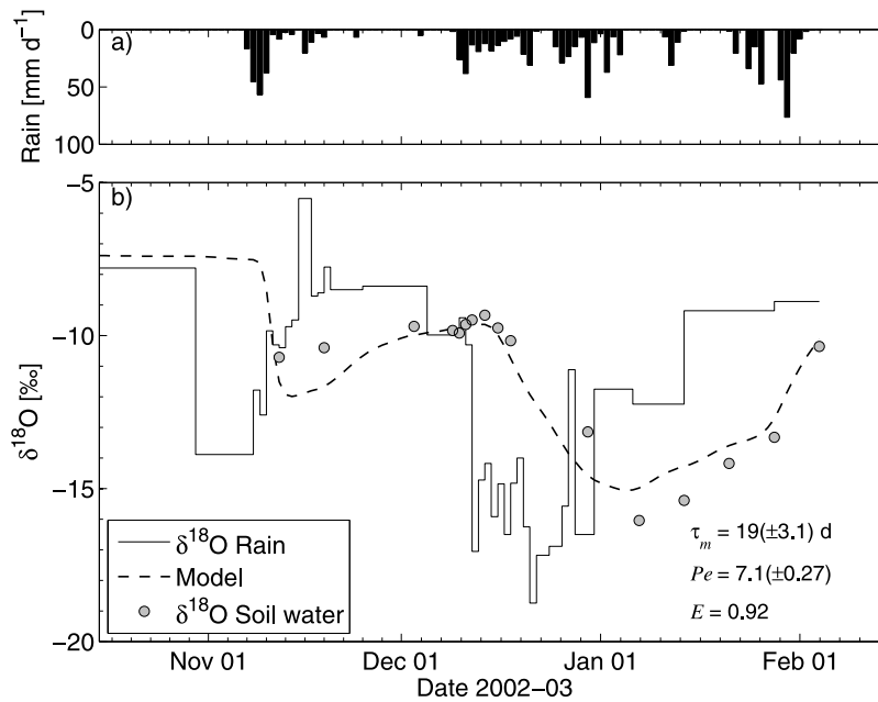
Figure 9. (a) Daily rainfall and (b) an example \delta^{18}\text{O} simulation for lysimeter D70 modeled using a one-dimensional advection-dispersion model. The mean transit time ( \tau_m ) for this simulation is 19 (\pm 3.1) days with a Peclet number, Pe , ( 1/D_p ) of 7.1 (\pm 0.27) (i.e., a fitting parameter describing ratio of advective to dispersive time scales). The Nash-Sutcliffe efficiency [Nash and Sutcliffe, 1970], E , is 0.92. The analytical precision of \delta^{18}\text{O} (0.11‰) is less than the size of the plotted circle for soil water \delta^{18}\text{O} .
