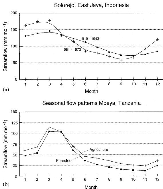
Fig. 5. (a) Change in seasonal distribution of streamflow following changes in land use: replacing 33% of forest by rainfed cropping and settlements in East Java, Indonesia (after Rijdsdijk and Bruijnzeel, 1991). (b) Change in seasonal distribution of streamflow following changes in land use: replacing montane rain forest by subsistence cropping in Tanzania (based on original data in Edwards, 1979).
