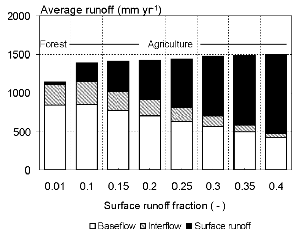
Fig. 6. Simulated changes in streamflow components for forested and agricultural conditions with increasing soil disturbance (after Van der Weert, 1994).
