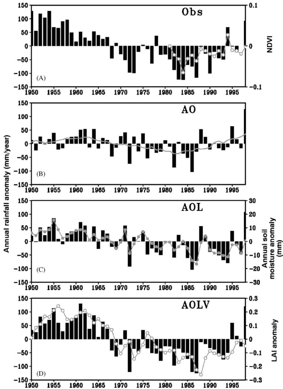
Fig. 1. Annual rainfall anomaly (vertical bars) over the West African Sahel ( 13\text{--}20^{\circ}\text{N} , 15^{\circ}\text{W}\text{--}20^{\circ}\text{E} ) from 1950 to 1998: (A) observations; (B) model with non-interactive land-surface hydrology (fixed soil moisture) and non-interactive vegetation (SST influence only; AO). Smoothed line is a 9-year running mean showing the low-frequency variation. (C) Model with interactive soil moisture but non-interactive vegetation (AOL); (D) model with interactive soil moisture and vegetation (AOLV) (after Zeng et al., 1999).
