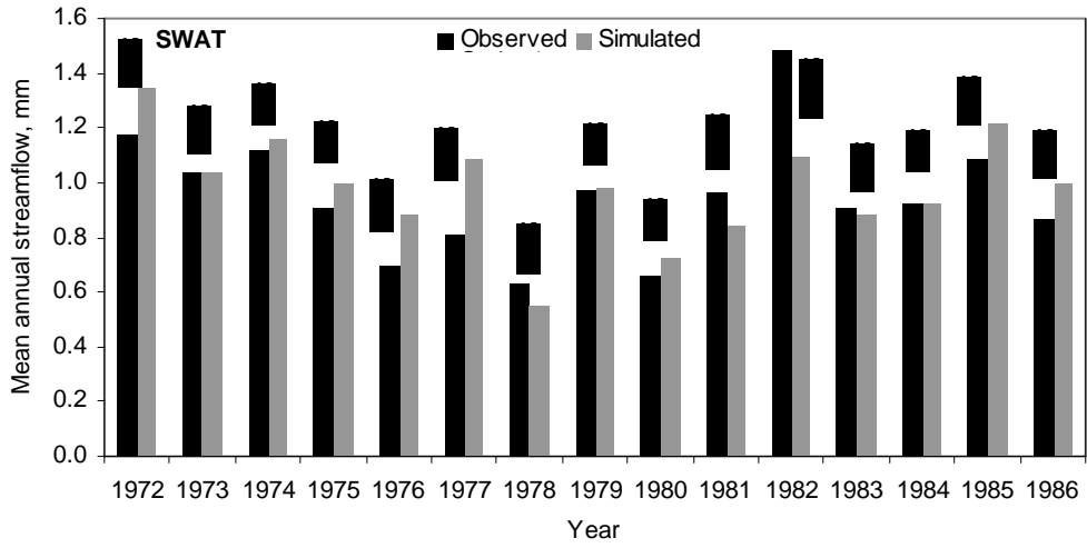
Figure 5. Comparison of observed and simulated annual streamflows and their percent errors for HSPF and SWAT for model verification period of 1972-1986
