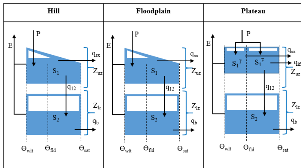
Figure 8: FUSE_TOPO_M1 model configuration (P: precipitation, E: evaporation, q_b : base flow, q_{sx} : surface flow, q_{12} : percolation, q_{if} : interflow, Z_{uz} and Z_{lz} : depth of unsaturated zone and saturated zone, S_1 and S_2 : total water content in the unsaturated zone and saturated zone, S_1^F : free water content in the unsaturated zone, S_1^T : tension water content in the unsaturated zone, \Theta_{wit} : soil moisture at the wilting point, \Theta_{fld} : soil moisture at field capacity, \Theta_{sat} : soil moisture at saturation)
