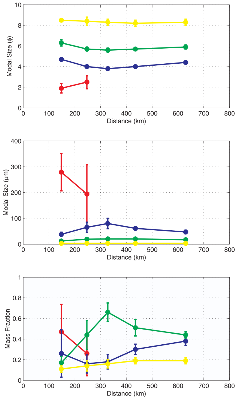
Figure 11. Particle subpopulations in MSH80 fallout averaged by transect as a function of distance from Mount St. Helens. Modes in units of (top) \Phi and (middle) \mu\text{m} . Overall average modes are located at 2.2 \Phi ( 237 \mu\text{m} ), 4.2 \Phi ( 58 \mu\text{m} ), 5.8 \Phi ( 19 \mu\text{m} ), and 8.3 \Phi ( 3 \mu\text{m} ). (bottom) The proportion of each subpopulation as a function of distance. There is an enhancement in the proportion of the subpopulation with a mode at 5.8 \Phi ( 19 \mu\text{m} ) over the distal mass deposition maximum.
