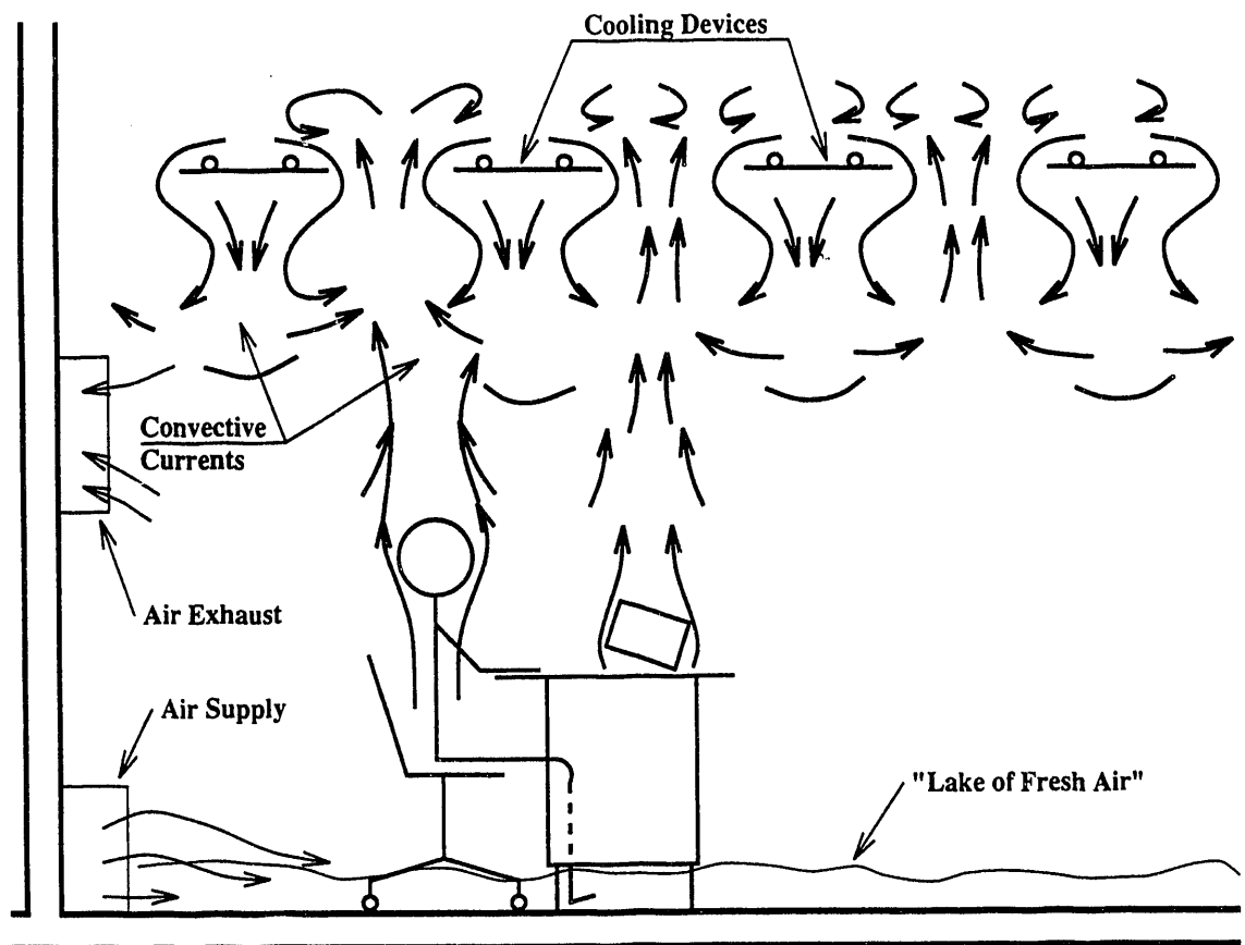
Figure 2: Air Flow Patterns in a Room with a Cooled Ceiling [18]
