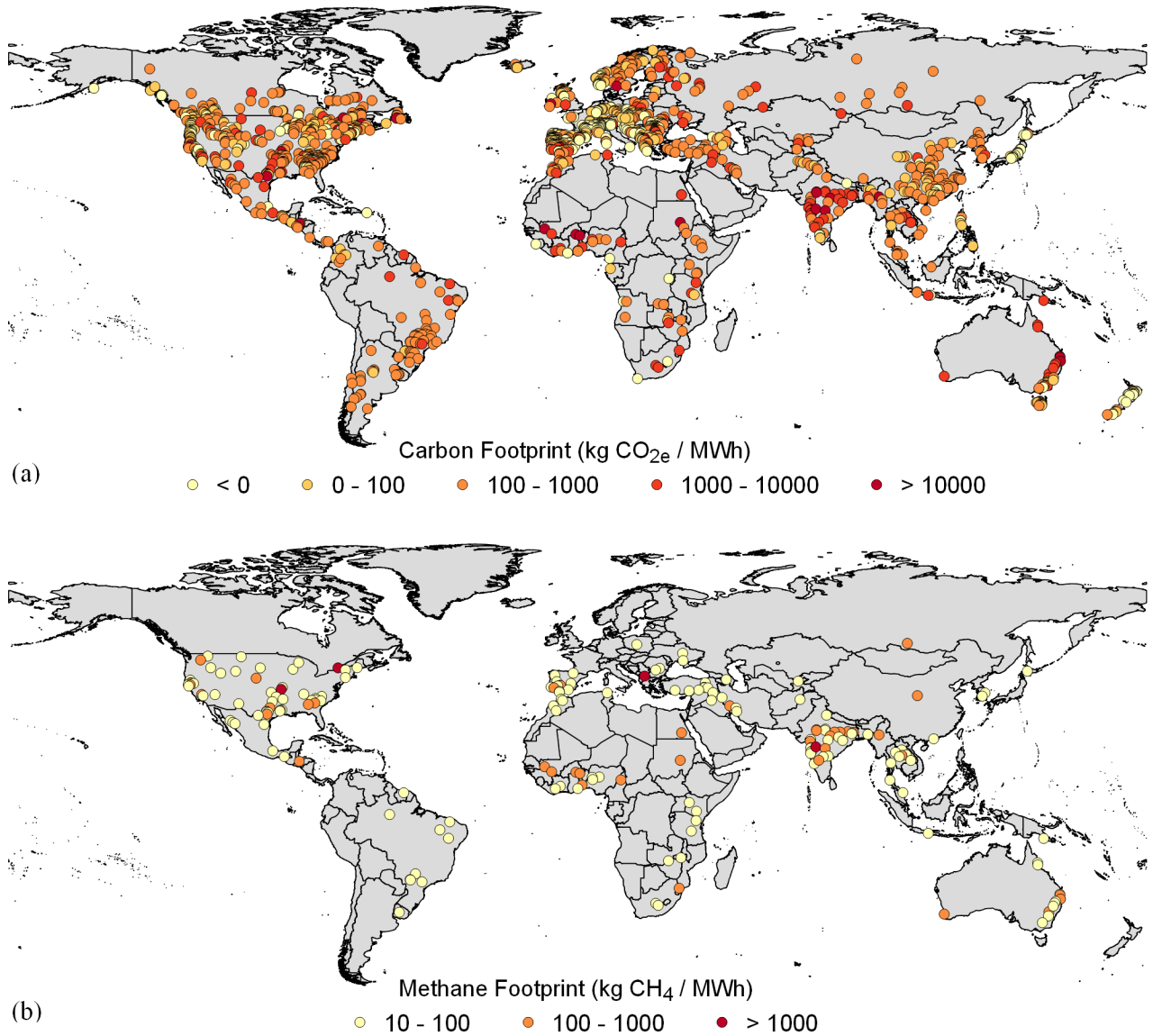
Fig 1. Carbon footprints of hydropower plants across the world (a) and hydropower plants with high methane emissions ( \geq 10 kg CH 4 /MWh) and a large share of methane emissions ( \geq 50\% of the carbon footprint) (b). Country boundaries are obtained from Natural Earth ( http://www.naturalearthdata.com/ ).
