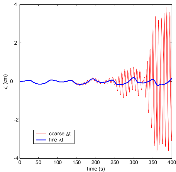
Figure 4.1: Scenario 6 pycnocline displacement simulated with a coarse timestep, determined by CFL_x , and a fine timestep, determined by CFL_z .
