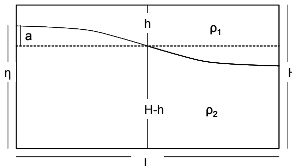
Figure 3.9: Schematic of basin.
