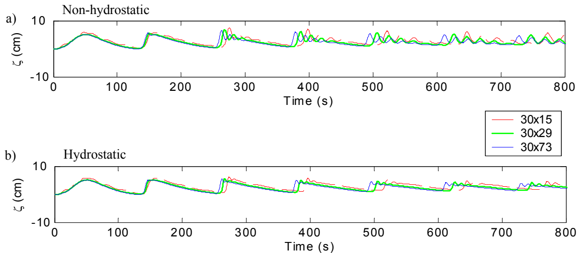
Figure 4.7: Isopycnal displacement of scenario 2 for vertical grid refinement, measured at the center of basin. a) Non-hydrostatic model, b) hydrostatic model.
