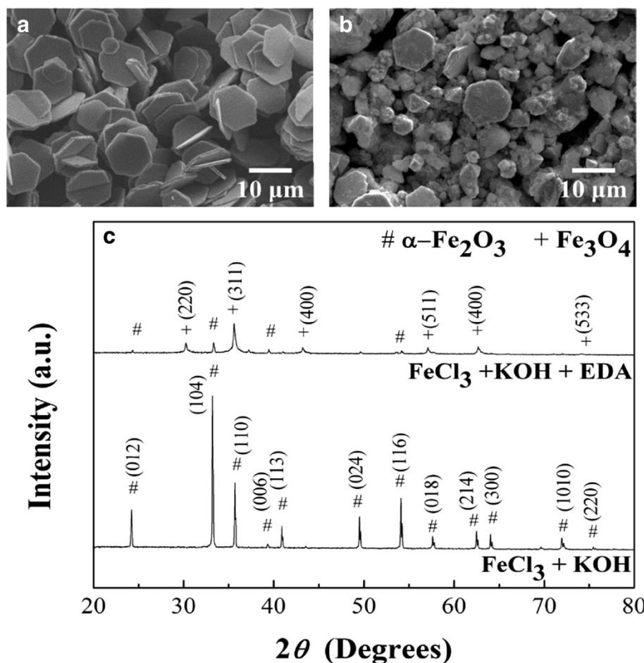
Figure 5 SEM images and corresponding XRD patterns of iron oxide particles. SEM images of iron oxide particles formed with (a) FeCl 3 + KOH and (b) FeCl 3 + KOH + EDA. (c) The corresponding XRD patterns of iron oxide obtained for the cases of (a) and (b).
