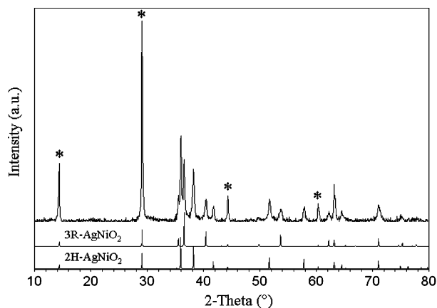
Figure 9. The PXD pattern of the \text{AgNiO}_2 product consists of a mixture of both the 00 l -ordered (*) 2H- and 3R-polytypes. Calculated positions, both indexed and indicating relative intensities, are shown for 2H- \text{AgNiO}_2 and 3R- \text{AgNiO}_2 (JCPDS #49-0666).
