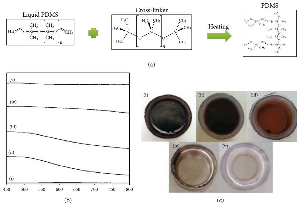
FIGURE 4: Dependence of the cross-linking degree on the incorporation of gold (Au) nanoparticles in the PDMS film surface modification. (a) General reaction between the cross-linker and liquid PDMS, (b) UV-visible absorption spectra, and (c) photographs of the Au-PDMS composite films containing (i) 2, (ii) 4, (iii) 6, (iv) 8, and (v) 10 wt% of the cross-linker to liquid PDMS. Reprinted with permission from [145], M. Tagaya et al., Smart Materials Research . 2011, 1–7 (2011) © 2011, Hindawi.
