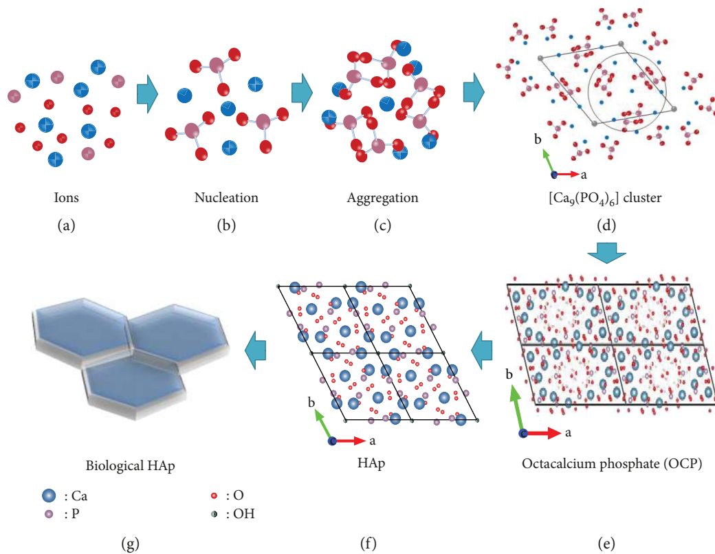
FIGURE 8: Scheme of the biomineralization process. (a) Ions in solution, (b) nucleation, (c) aggregation, (d) amorphous calcium phosphate—the circle shows the Posner cluster unit [Ca_9(PO_4)_6] projected on the ab plane, (e) octacalcium phosphate, projected on the ab plane, (f) hydroxyapatite projected on the ab plane, and (g) biological hydroxyapatite [199–202] (drawing using VESTA (10) from the CIF obtained from American Mineralogist Crystal Structure Database).
