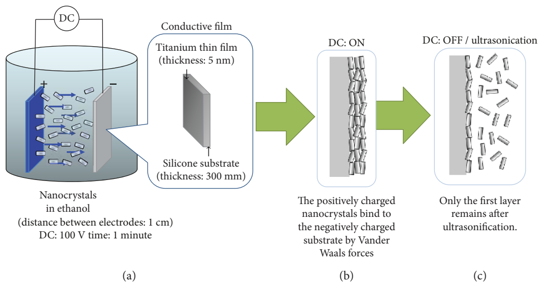
FIGURE 6: (a) Scheme of the electrophoretic deposition (EPD) procedure with a direct current (DC) of 100 V, (b) deposition mechanism in ethanol, and (c) resultant electrophoretic deposition system at the monolayer, after ultrasonification. Reprinted with permission from [190], M. Tagaya et al., Sci. Technology Adv. Mater. 92 11 045002.1–045002.8. (2010) © 2010 IOP Publishing.
