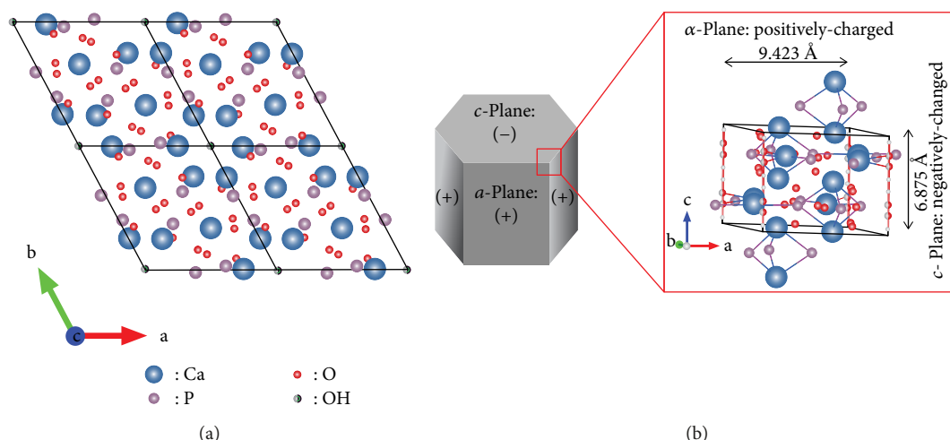
FIGURE 1: (a) Crystal structure of HAP in the top view along with the c -axis, which were centered on the hexagonal c -axis channel and (b) the overview structure to exhibit the rich phosphate and hydroxyl ions at the c -plane and the calcium ions at the a -plane (drawing using VESTA (10) from the CIF obtained from American Mineralogist Crystal Structure Database).
