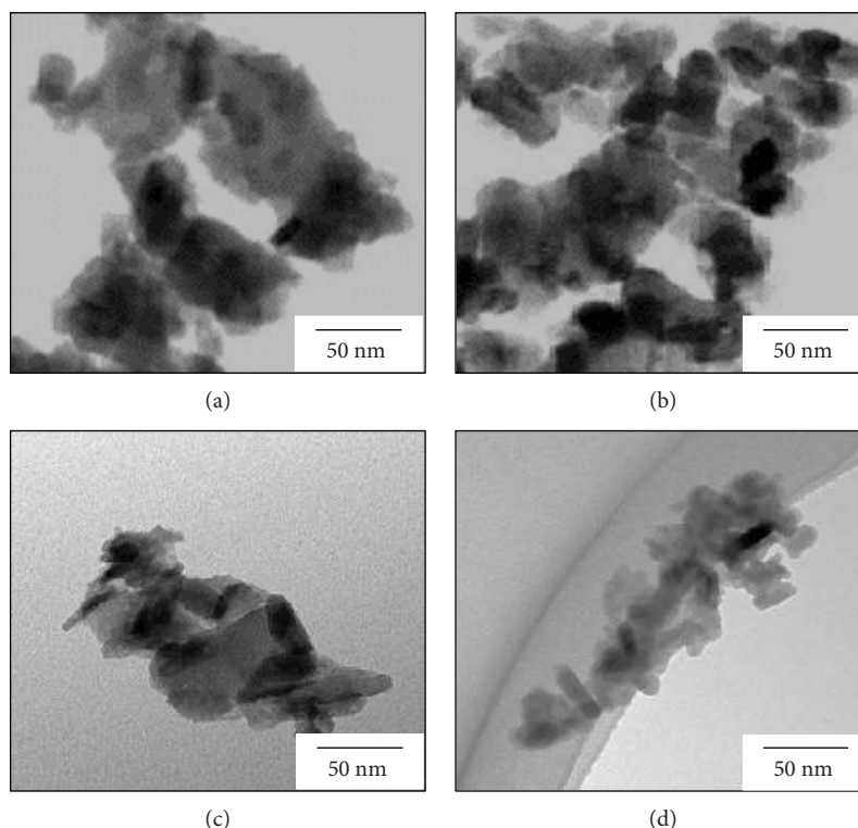
FIGURE 2: TEM images of (a) general HAp (HAp-40-Aft) NPs, (b) cationic surfactant-assisted HAp (CTAB/HAp-40-Aft) NPs, (c) zinc ion-doped HAp (0.5-Zn:HAp) NPs, and (d) zinc ion-doped CHAp (0.5-Zn:HAp) NPs. Reprinted with permission from [57], K. Shiba et al., Cryst. Growth Des. 16, 1463–1471 (2016) © 2016, American Chemical Society, and [68] T.G.P. Galindo et al., J. Nanomater. 2015, 360 (2015) © 2015, Hindawi.
