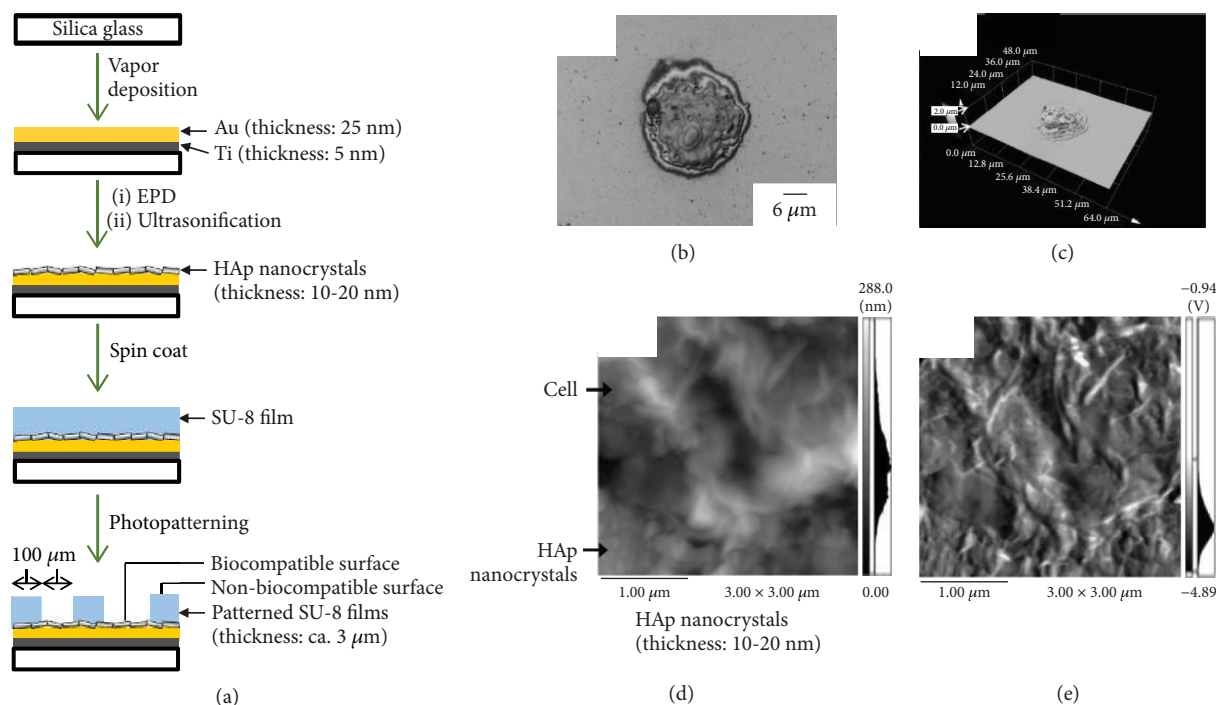
FIGURE 10: Study of hepatocyte cell aggregation and adhesion at HAP NPs covered with SU-8 polymer micropatterns by nano/microfabrication techniques. (a) Schematic illustration of the micropatterning process to obtain SU-8/HAP nanocrystals/Au/Ti/silica substrate and the subsequent cells adhered on HAP surface, (b) optical microscopic image of a cell, (c) 3D graphics image of the cell, (d) AFM topographic, and (e) phase shift images of the cell and HAP nanocrystalline surfaces. Reprinted with permission from [239], M. Tagaya et al., Macromol. Biosci. 11, 1586–1593 (2011) © 2011, Wiley-VCH.
