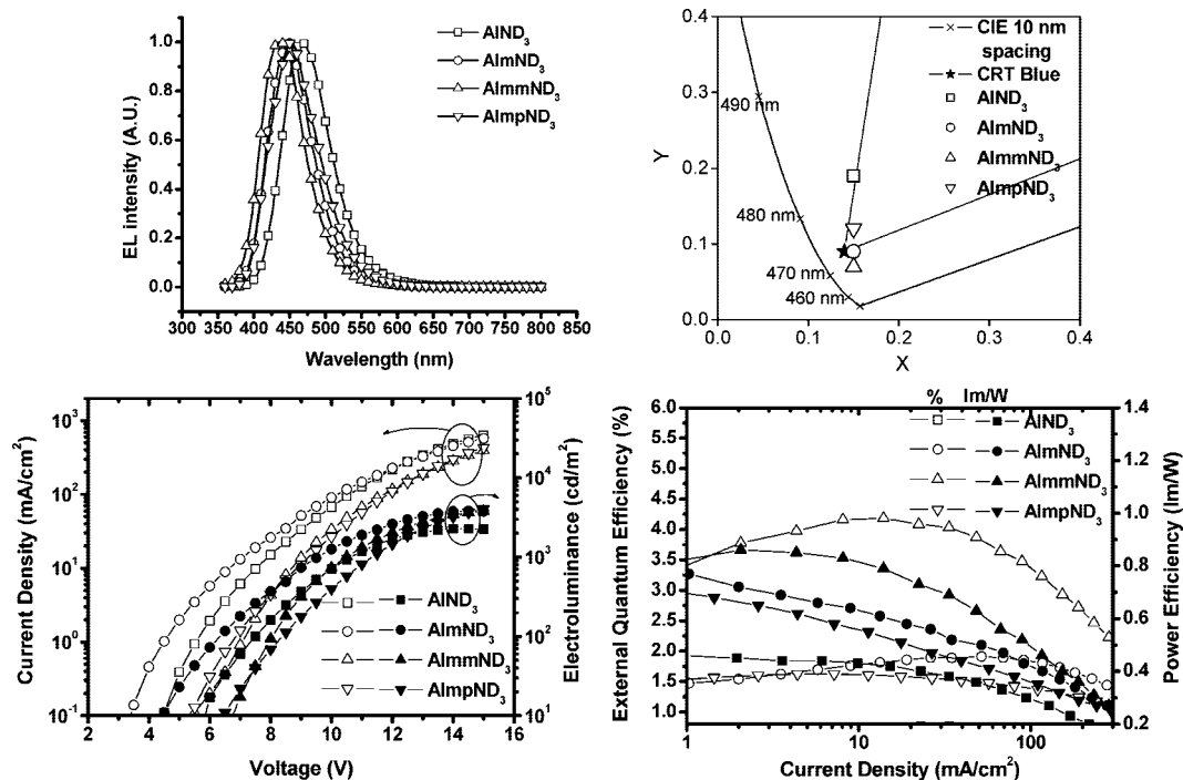
Figure 10. EL characteristics of ITO/NPB(40 nm)/CBP(10 nm)/Blue Al chelate(30 nm)/ETL(20 nm)/LiF(0.5 nm)/Al(150 nm), where Blue Al chelate is \text{AImND}_3 , \text{AlmND}_3 , \text{AlmmND}_3 , and \text{AlmpND}_3 , respectively.
