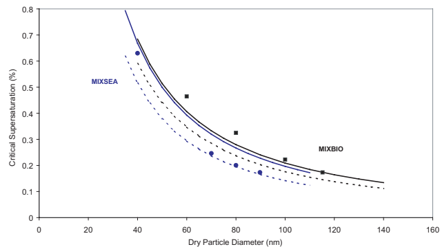
Fig. 5b. Critical supersaturation as a function of particle diameter for the mixtures MIXBIO and MIXSEA. Calculated critical supersaturations are represented by solid lines. The calculations are based on the parameterization of water activity (Table 4) and the surface tension (Table 3). The dotted blue line is obtained using a parameterization for MIXSEA, based on ZSR mixing rule (solid blue line, Fig. 3b). The dotted black line is obtained using Raoult's law and the ZSR mixing rule as described in section about MIXPO.
