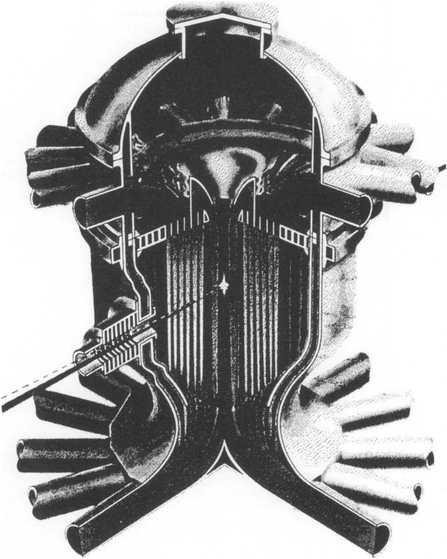
FIGURE 3 HYLIFE-I used steady flow.
