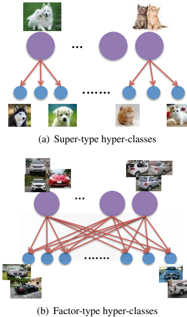
Figure 2. Two types of relationships between hyper-classes and fine-grained classes.
