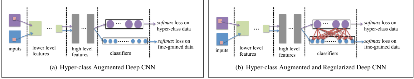
Figure 4. The network structures.
