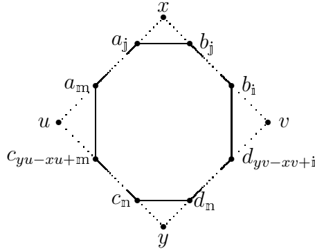
Figure 6: A chordless cycle in \mathcal{Q}(x, u, y, v) .
