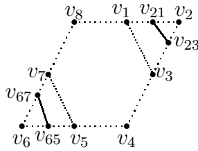
Figure 9: \mathbb{G}_{6(2t+1)}^q .
