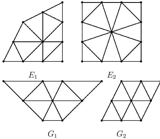
Figure 2: Four bridged graphs with hyperbolicity 1.
