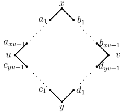
Figure 3: The geodesic quadrangle \mathcal{Q}(x, u, y, v) .
