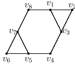
Figure 7: The outerplanar graph F_2 has chordality 6, hyperbolicity \frac{3}{2} , and tree-length 2.
