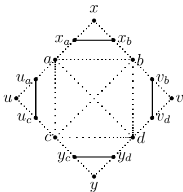
Figure 8: \mathbb{G}_{4t}^q .
