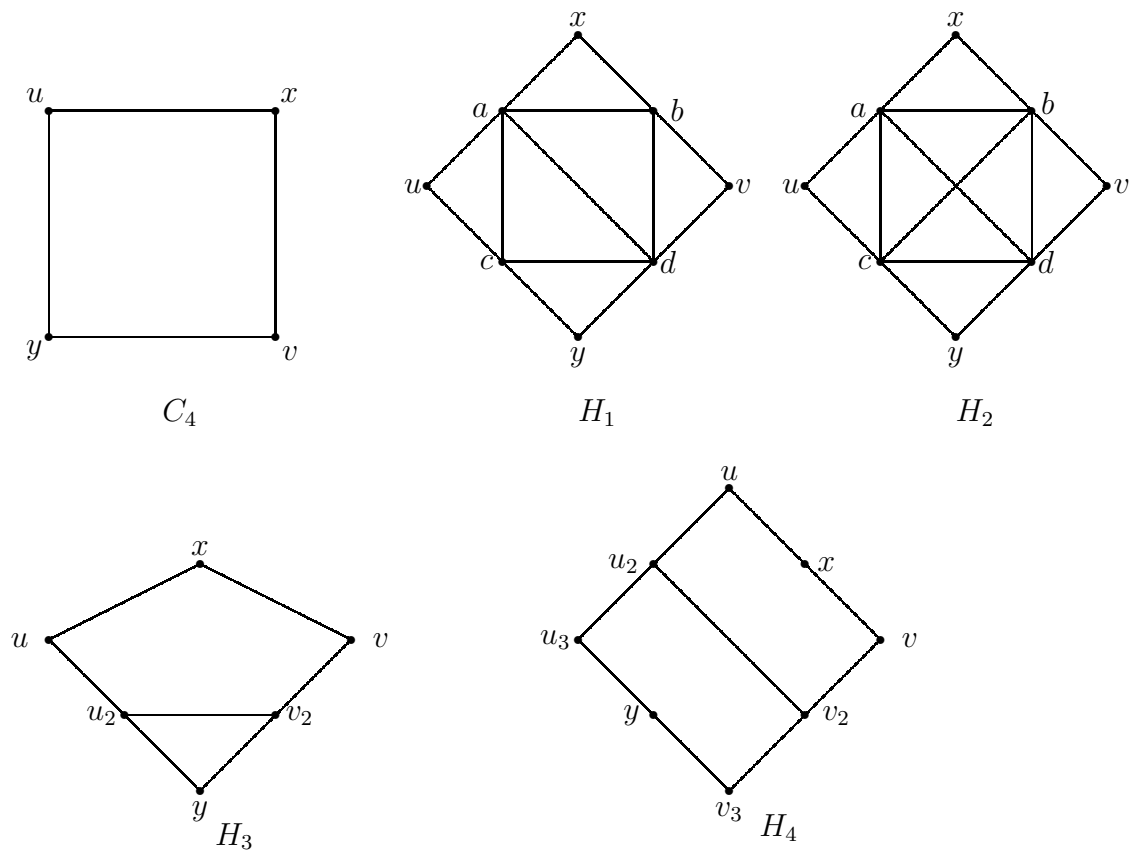
Figure 1: Five 5-chordal graphs with hyperbolicity 1.
