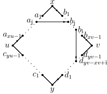
Figure 5: xy \leq i + b_i d_{yv-xv+i} + (yv - (xv - i)) , uv \leq (xu - j) + a_j b_j + (xv - j) .
