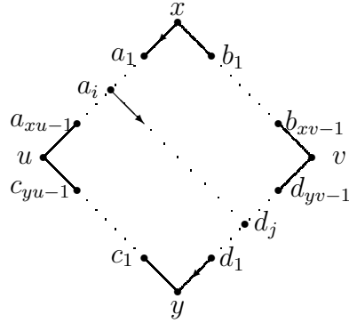
Figure 4: xy \leq i + a_i d_j + j .
