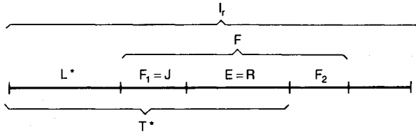
Fig. 3. The intervals L_r, T^*, L^*, F_i and E
