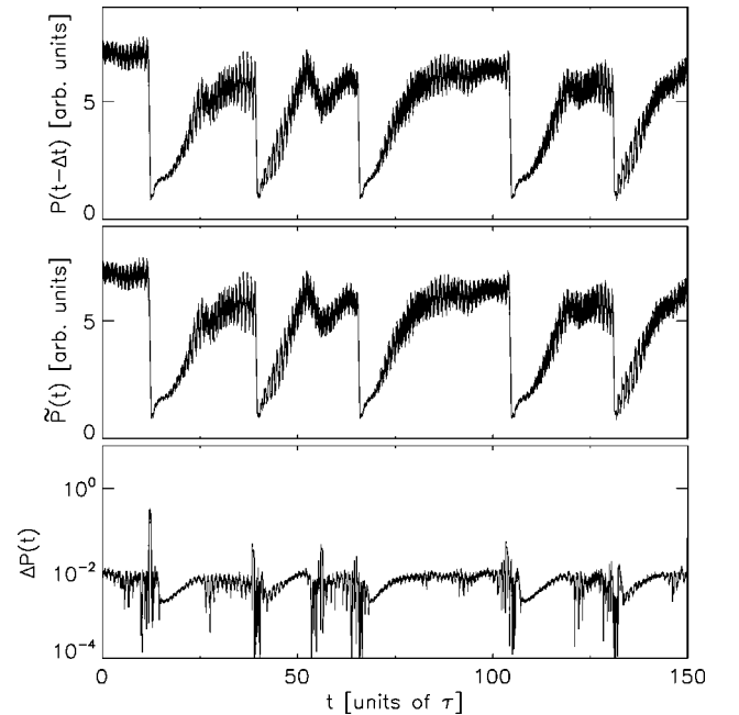
FIG. 9. Same parameters as in Fig. 7 but intensities P(t) = E_0^2(t) averaged over 5 ns to take into account finite detection time. Note that P(t - \Delta t) is plotted including the time shift \Delta t to demonstrate the simultaneous occurrences of the intensity breakdowns.
