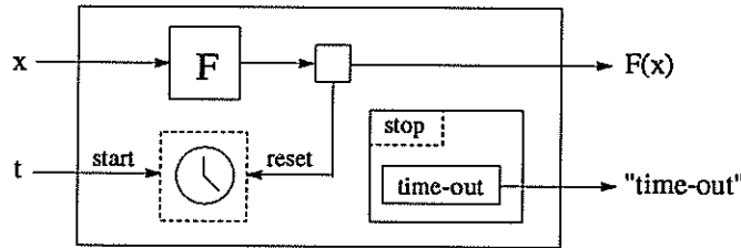
Figure 9: Function Evaluation with Time-out
