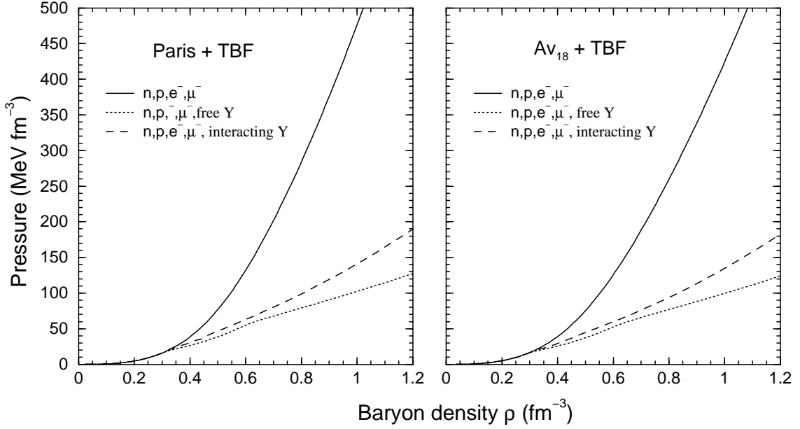
FIG. 7. As Fig. 4, but including three-body forces.
