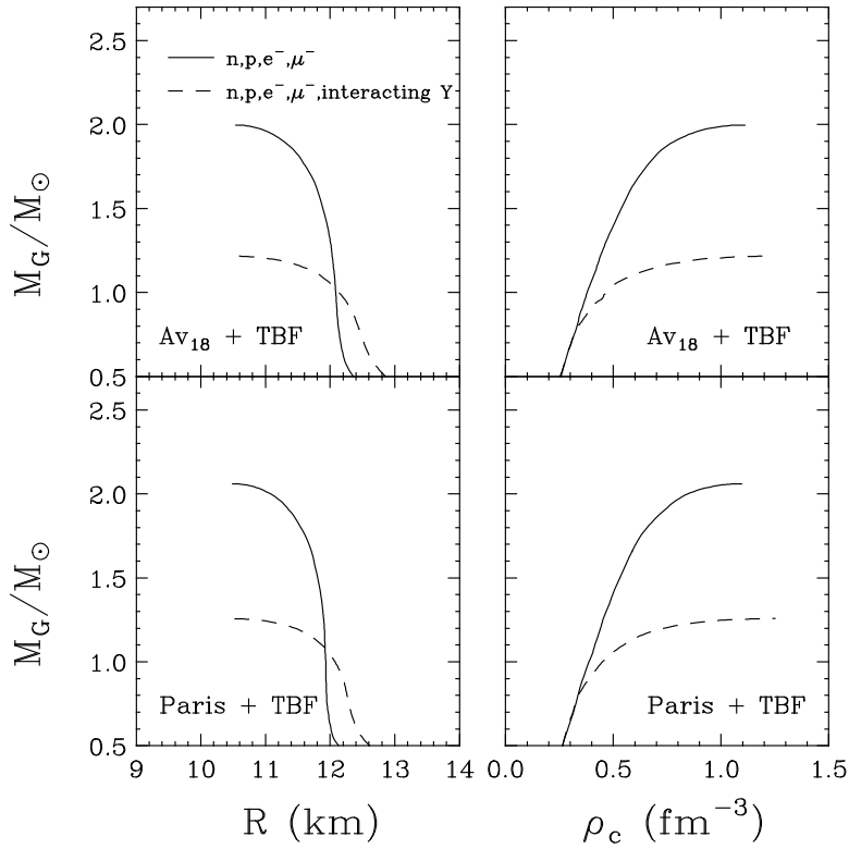
FIG. 9. Neutron star mass as a function of radius (left) or central baryon density (right) in the BHF+TBF model. Results without (solid lines) and with interacting hyperons (dashed lines) are compared.
