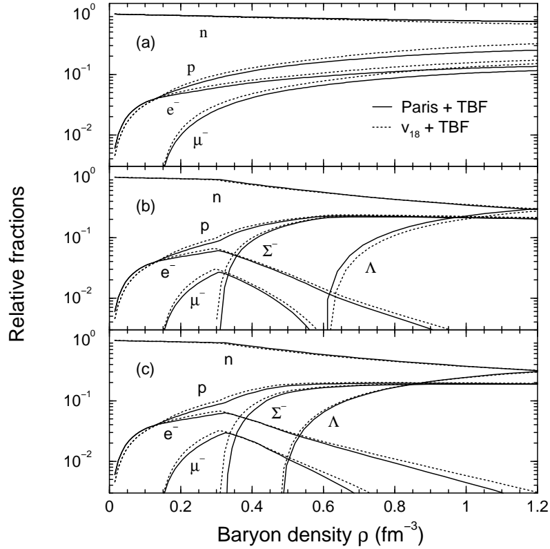
FIG. 6. As Fig. 3, but the nucleon-nucleon potentials are supplemented by three-body forces.
