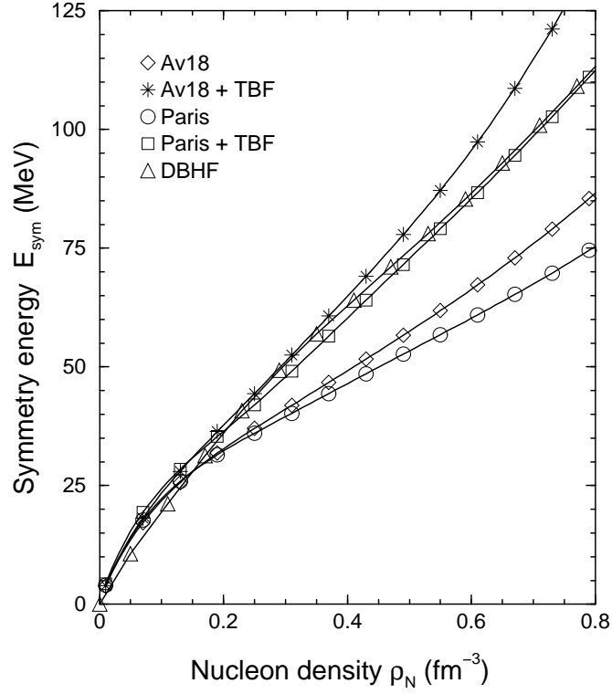
FIG. 5. Nucleonic symmetry energy as a function of nucleon density obtained in different theoretical models of nuclear matter.
