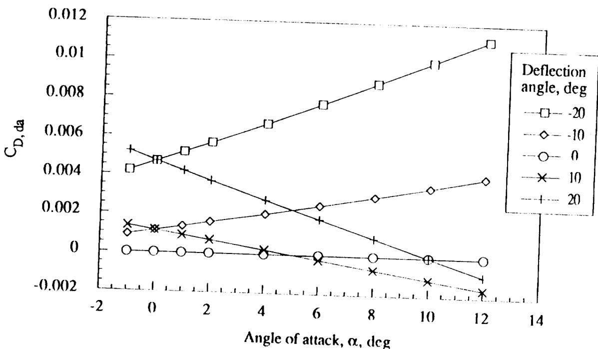
(e) Mach number = 2.5
