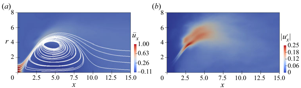
Figure 7. Time-averaged flow structure of regular conical form of vortex breakdown (CVB) at S = 1.8 on meridional plane: (a) projected streamlines overlaid on contours of mean axial velocity and (b) rms of the fluctuating axial velocity component.
