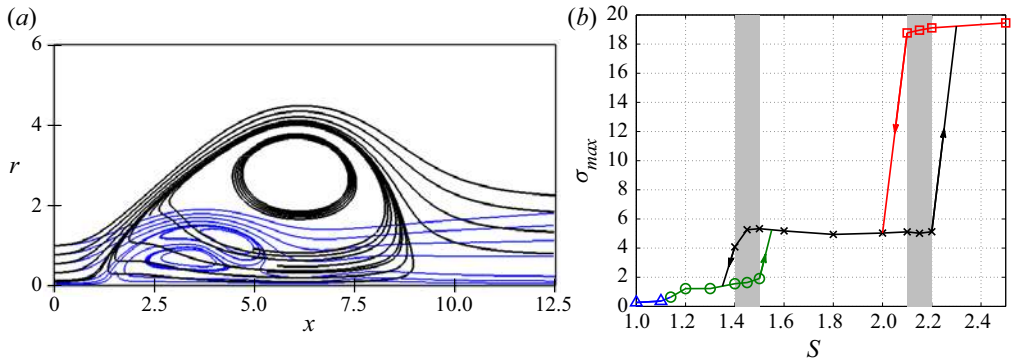
Figure 12. (a) Comparison of time-averaged flow features using projected streamlines on meridional plane for bistable forms at S = 1.4 : ———, blue (thin), bubble form of vortex breakdown (BVB); ———, black (thick), conical form of vortex breakdown (CVB). (b) A hysteresis curve based on maximum radial extent of a streamline starting from x = 0 and r = 0.2 , both obtained as swirl rate, S , is varied for Re = 1000 (regions of overlap shaded grey): ( \Delta , blue), pre-VB; ( \circ , green), oscillating BVB; ( \times , black), regular CVB; ( \square , red), wide-open CVB.
