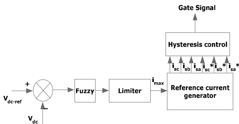
Figure 7. Conventional fuzzy controller.
