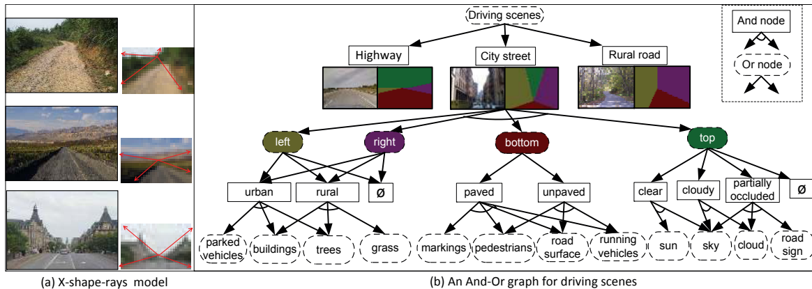
Fig. 27. (a) Under a low resolution (e.g. 32 \times 32 pixels), a driving scene can be approximated by a X-shape-rays model with four components (left, right, bottom and top). (b) The AoG used for parsing driving scenes. \Phi means a component is missing.
