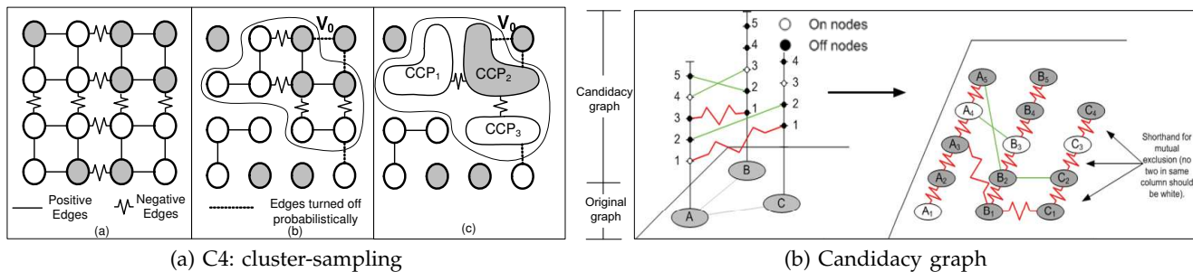
Fig. 14. (a) A visualization of the C4 algorithm. Here negative edges down the center encourage the four corners to be opposite colors, creating a checkerboard pattern. The right panel shows a connected component V_0 formed after edges are turned on and off. V_0 can be broken down in the final panel into subcomponents of like-colored nodes connected by negative edges. (b) Conversion from a candidacy graph to a binary graph with positive/negative edges. From [51].
