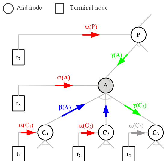
Fig. 12. Illustration of identifying the \alpha(A) , \beta(A) and \gamma(A) inference process for node A in an AoG (see text for detail definitions). The \alpha(A) process is directly based on the compact image data of node A (either bottom-up or top-down), the \beta(A) process generates hypotheses of node A by bottom-up binding the \alpha processes of some child node(s) (e.g. (\alpha(C_1), \alpha(C_2)) \rightarrow \beta(A) ), and the \gamma(A) process predicates hypotheses of node A from the \alpha processes of some parent node(s) (e.g. \alpha(P) \rightarrow \gamma(A) in a top-down fashion). In computing, each process has two states: “on” or “off”. For example, the \alpha process of node C_3 is off and we show it in grey. Because AoG is often recursively defined, each node has its own \alpha , \beta and \gamma processes. Modified from [64].
