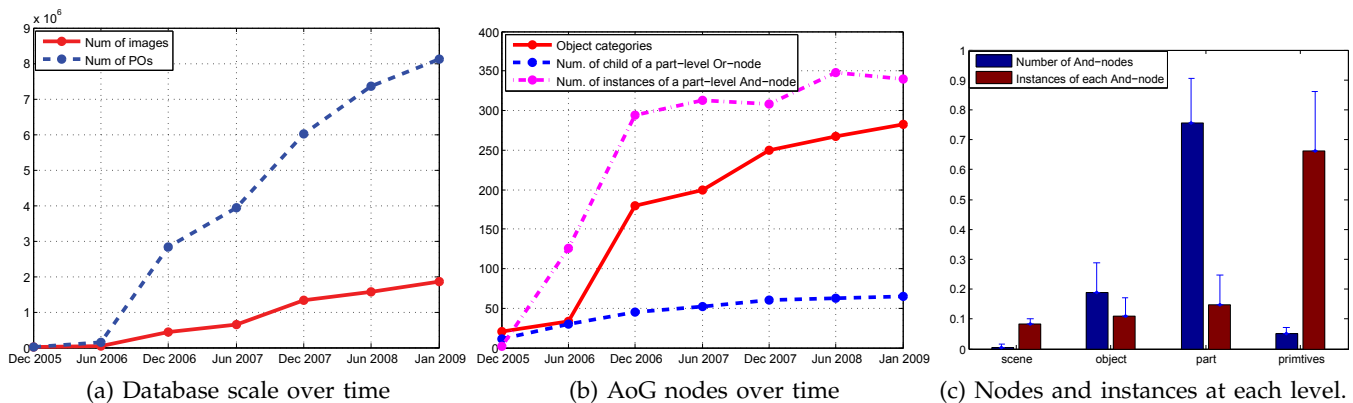
Fig. 11. Statistics of the LHI database. (a) Number of annotated images and POs over time. (b) Number of object categories over time, average number of children of a part-level Or-node and average number of instances of a part-level And-node over time. (c) Average number of And-nodes and instances at “scene”, “object”, “part” and “primitive” levels respectively (estimated from 20 object categories and normalized to 1).
