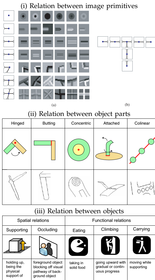
Fig. 8. Examples of three types of relations in the AoG. Modified from [36]
