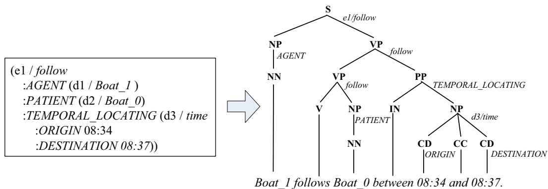
Fig. 23. An example of functional description (FD) of a video event being converted to natural language text by the text realizer. The FD is first transformed to a part-of-speech tree (POS) where additional syntactic terms (“between” and “and”) are inserted. The POS tree is then linearized to form a sentence. Notice that the FD and the POS tree share similar hierarchical structure, but there are notable differences. In the FD, children nodes are unordered. In the POS tree, the ordering of children nodes is important and additional syntactic nodes are inserted.
