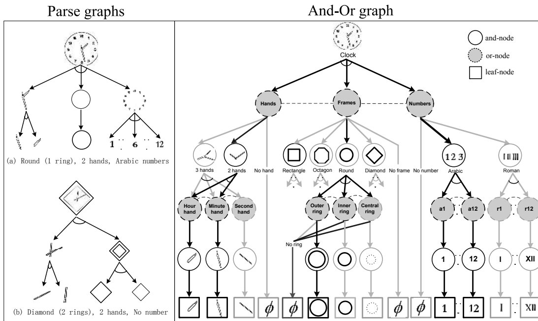
Fig. 4. Categorical representation with AoG. The left panel illustrates two parse graphs of clocks. The right panel shows an AoG of a clock generated from merging multiple parse graphs together. The dark arrows in the AoG illustrate one parse graph (a round clock). Some leaf nodes are omitted from the graph for clarity. Edited from [36].
