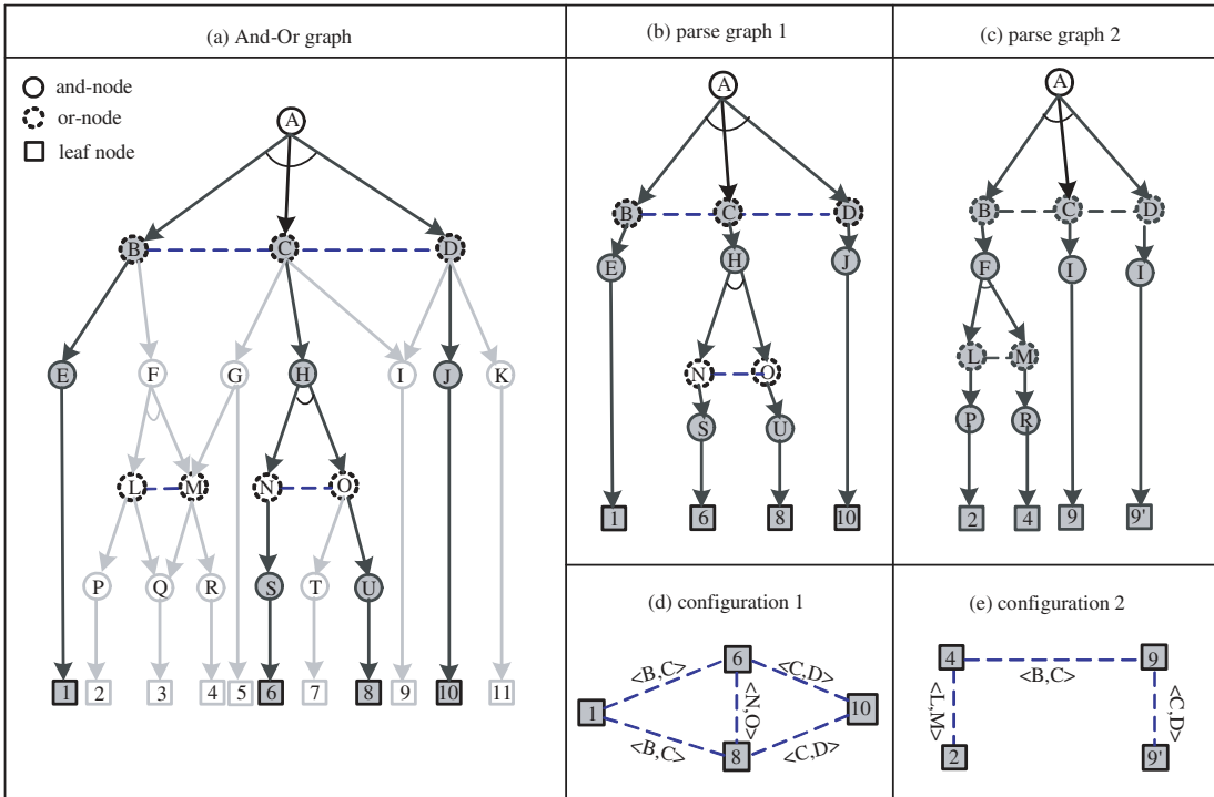
Fig. 5. Illustrating the AoG representation. (a) An AoG embodies the grammar productions rules and contexts. It contains many parse graphs, one of which is shown in bold arrows. (b) and (c) are two distinct parse graphs obtained by selecting the switches at related Or-nodes. (d) and (e) are two graphical configurations produced by the two parse graphs, respectively. The links of these configurations are inherited from the AoG relations. From [36].
