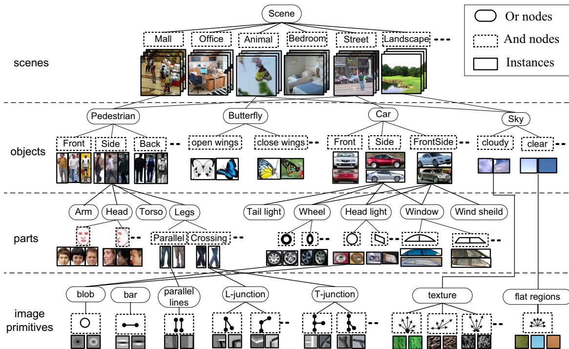
Fig. 9. Visual vocabularies of scenes, objects, parts and image primitives compiled into an AoG representation. Each Or-node (solid ellipses) represents for a visual concept and is pointed to alternative subconfigurations. Each And-node (dashed rectangles) is associated with a set of instances (solid rectangles) from an annotated image database and can be decomposed into a number of components in a lower level. Please see text for detailed discussion of each dictionary. For clarity purposes, only part of the vertical links are shown.
