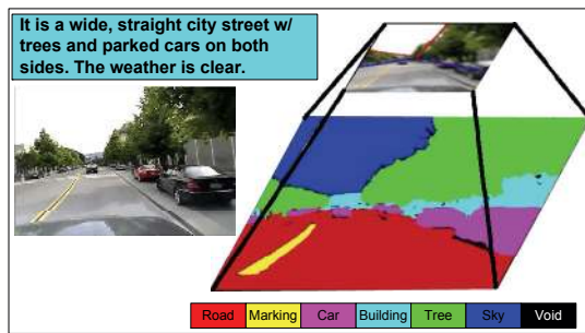
Fig. 28. An example of parsing and text generation results.
