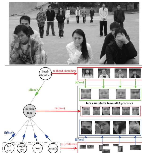
Fig. 13. Illustration of integrating the \alpha(face) , \beta(face) and \gamma(face) in the human face AoG for face detection. The three inference processes are effective in complementary ways depending on the scale and occlusion conditions. The typical situations shown here are common to other object categories. Modified from [64].
