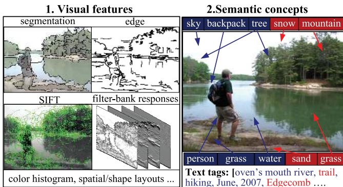
Fig. 3. Categorical representation of visual contents. Task1. Extract low level visual features from raw images. Task2. Map visual features into semantic concepts. Concepts in blue color are correct ones that are related to the image content. Concepts in red are irrelevant, and are generated by either classification error or unrelated text tags.
