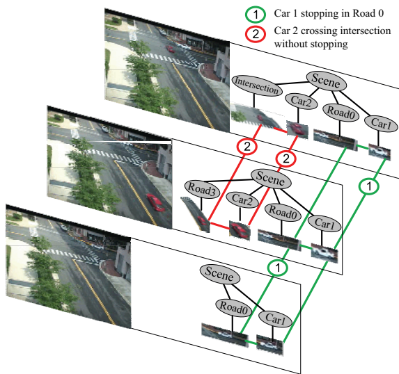
Fig. 25. An example of video event detection involving a failure-to-yield incident. Each image frame is represented by a parse graph and objects are tracked over frames. In the event grammar, complex events are composed of elementary events observed as the motion of objects (cars) with respect to scene context (road lanes and intersection). There are two events in this example: (1) Car-1 stopping in Road-0. (2) Car-2 crossing intersection without stopping.
