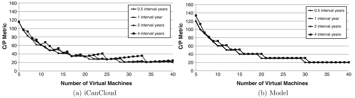
Fig. 10 Simulation versus mathematical model of Phobos using high CPU medium instances
