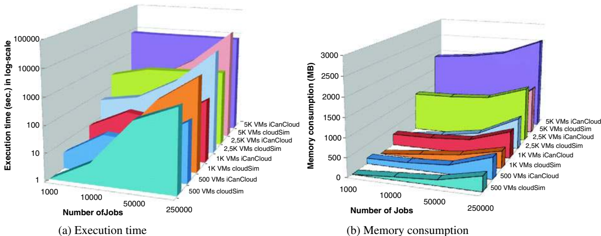
Fig. 13 Performance experiments: iCanCloud versus cloudSim
