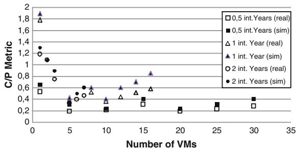
Fig. 12 Simulation versus Amazon EC2 execution of Phobos using small instances
