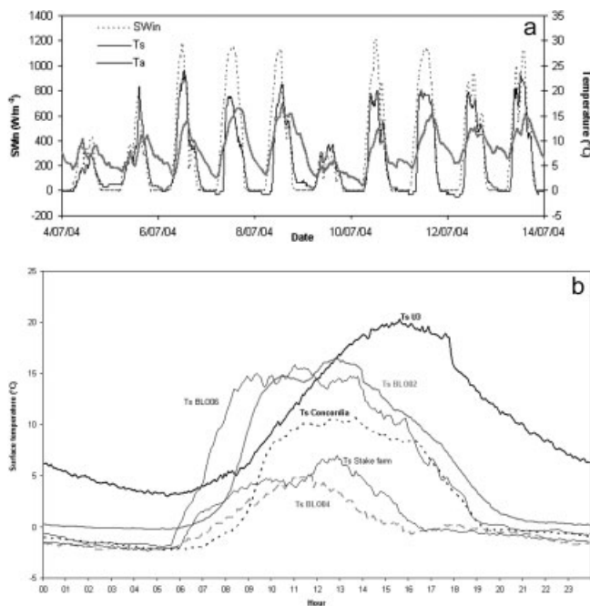
Fig. 9. (a) Estimated debris surface temperature compared with the air temperature (calculated using Urdukas data and the calculated lapse rate) and incoming shortwave radiation ( \text{SW}_{in} ( \text{W m}^{-2} )) at Baltoro longitudinal profile 2 (mean altitude 4162.1 m). Dates are dd/m/yy. (b) Estimated surface temperature for different debris thicknesses (U3: 36 cm; BLO02: 11 cm; BLO06: 10 cm; Concordia: 4 cm; stake farm: 2 cm; BLO04: 1 cm) at different sample sites along the longitudinal profile from Urdukas to Concordia. Apart from Urdukas (U3, with north orientation), all the sites were located on flat surfaces.
