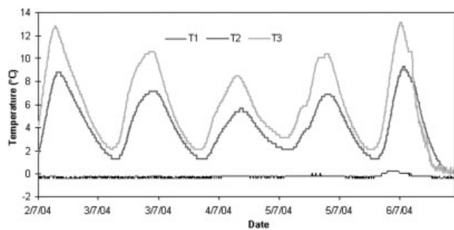
Fig. 8. Debris temperatures for different debris depths at Urdukas stakes. T1 is 36 cm from the surface at the buried ice contact, T2 20 cm and T3 13 cm from the surface. Dates are dd/m/yy.
