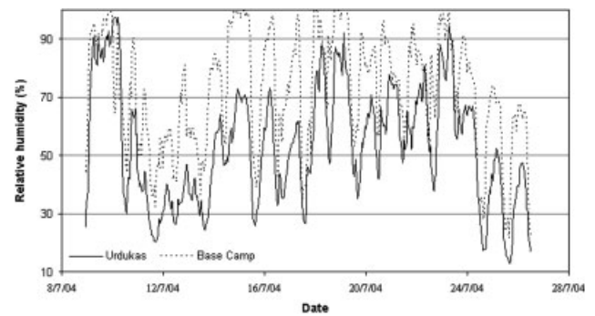
Fig. 3. Comparison between the mean hourly values of relative humidity (%) measured at the Urdukas and Base Camp AWSs. Dates are dd/m/yy.
