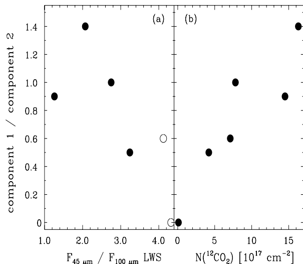
Fig. 14. The ratio of component 1 to component 2 as a function of the ratio of hot to cold dust a ) and the total \text{CO}_2 column density b ). Open symbols are for sources with unreliable (contaminated) 45/100 \mu\text{m} flux.
