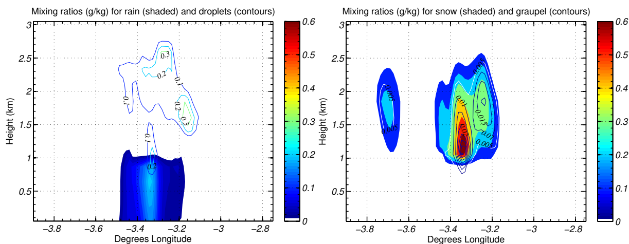
Fig. 9. Meridional cross-sections from model output at 51^\circ\text{N} at time 12:00 UTC. Left: liquid mixing ratios (rain and droplet categories); right: ice mixing ratios (snow and graupel categories). Plots are in units of \text{g kg}^{-1} .
