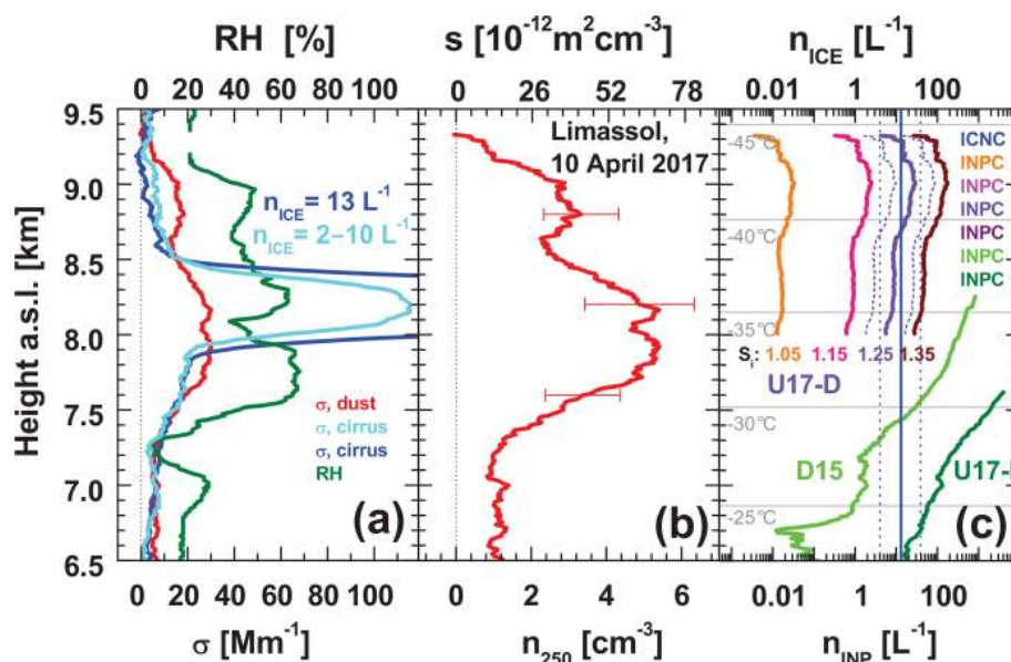
Figure 9. Cirrus INPC–ICNC closure study based on LACROS observations at Limassol, Cyprus, on 10 April 2017 (see Fig. 7) during CyCARE. (a) Dust extinction coefficient (06:10–06:30 UTC mean), ice crystal extinction coefficient (light blue, 06:35–06:42 UTC mean; blue, 06:48–06:57 UTC mean; cirrus from 8 to 8.5 km height), relative humidity (RH, radiosonde, launch at 05:50 UTC), estimated ICNC ( n_{ICE} : light blue for the 06:35–06:42 UTC time period; blue for the 06:58–07:05 UTC time period), (b) dust particle number concentration n_{250,d} (considering large particles with a radius of > 250 nm only) and surface area concentration s_d (06:10–06:30 UTC mean values), and (c) INPC ( n_{INP} , 06:10–06:30 UTC mean) determined by using the deposition nucleation U17-D(d) parameterization for four different ice supersaturation values ( S_i from 1.05 to 1.35). The uncertainty range of each of the four deposition nucleation INPC profiles is indicated for S_i = 1.10 . For comparison, also immersion freezing INPC profiles estimated by using the U17-I(d) (dark green) and D15 INP parameterizations (green, see Table 1) are shown. The ICNC value of 13 \text{ L}^{-1} (see the number in a) is shown as the vertical blue line with the uncertainty range as the vertical blue dashed lines.
