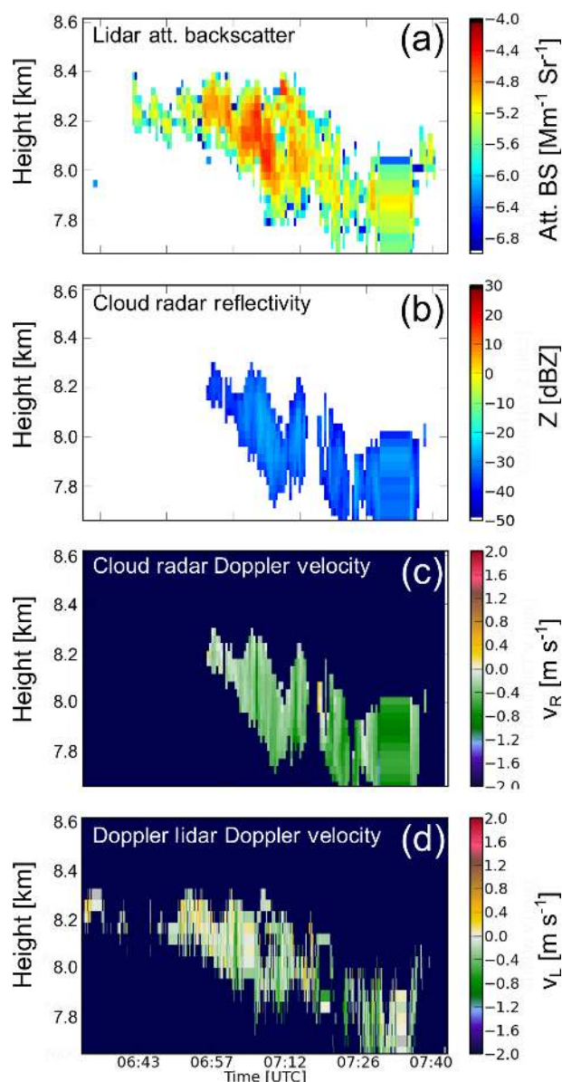
Figure 10. Evolution of a thin cirrus layer on 10 April 2017 (see also Fig. 7) as observed with Polly lidar in terms of (a) attenuated backscatter (at 532 nm), with cloud radar in terms of (b) radar reflectivity Z at 8.5 mm wavelength and (c) vertical velocity, v_R , and Doppler lidar in terms of (d) vertical velocity v_L .
