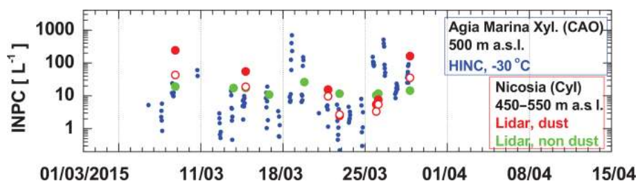
Figure 6. Comparison of in situ observations of the INPC (HINC, ETH Zurich; see the text for more explanation) at Agia Marina Xyliatou (about 500 m a.s.l.) and lidar-based INPC estimations (mean values for the 450–550 m a.s.l. height range) at Nicosia, about 25 km downwind of Agia Marina Xyliatou. All in situ observations collected in March 2015 are shown. The green circles indicate lidar estimates of the INPC based on the D10 parameterization (for non-dust continental aerosol pollution) and the red circles are computed by using the D15 parameterization (for the dust aerosol fraction). For comparison, we also include dust INPC values (open red circles) obtained with the D10(d) parameterization (see Table 1). All INPC values (HINC, lidar) are given for -30^{\circ}\text{C} .
