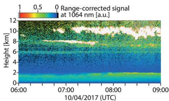
Figure 7. Development of a thin cirrus at 8 km height at 06:30 UTC on 10 April 2017. The thin cirrus layer was embedded in Saharan dust. An extended cirrus field is visible from 9 to 11 km height. The polluted boundary layer reached to about 2 km height. Ranged-corrected 1064 nm lidar signals are shown with 7.5 m and 30 s resolution.
