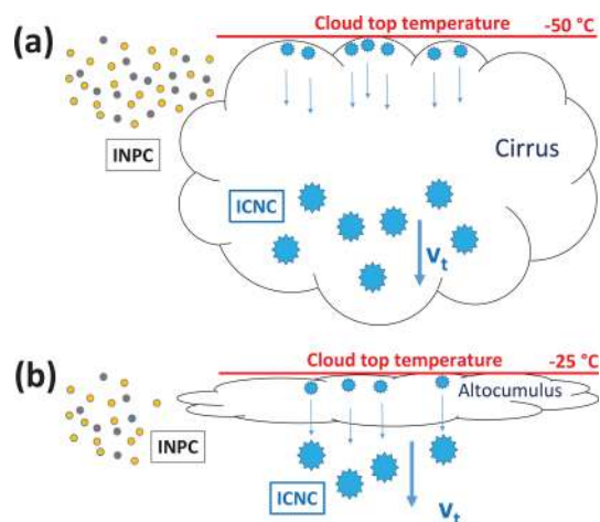
Figure 3. Illustration of the INPC–ICNC closure approach for (a) a vertically deep cirrus cloud and (b) a shallow stratiform mixed-phase altocumulus layer. In the first step, the INPC is retrieved from polarization lidar observations outside the cloud layer (e.g., before the cloud layer crosses the lidar field site). Gray and orange particles indicate continental pollution and mineral dust particles, respectively. In the second step, the ICNC is estimated from observations with the available backscatter lidar, Doppler lidar, and cloud radar instrumentations. Within the cirrus layer (a) the ICNC is preferably estimated in the lower part of the cloud with large ice crystals and thus clear falling features of ice crystals. v_t is the mean terminal velocity of the ice crystal population relative to the surrounding air. In the case of a shallow altocumulus layer (b), the ICNC is determined in the ice virga zone, below the main cloud layer in which backscatter by liquid droplets dominate the lidar return signals and prohibit ice observations. In the closure experiments, we assume that all ice crystals nucleate at the top of the cloud layer (at the coldest point of the cloud layer), grow quickly, and start falling and that the number of nucleated ice crystals does not change on the way downward towards the lower part of the cirrus (a) and below the altocumulus layer (b), i.e., that collisions of ice crystals and the subsequent formation of crystal aggregates as well as secondary ice production do not change the number of nucleated ice crystals significantly.
