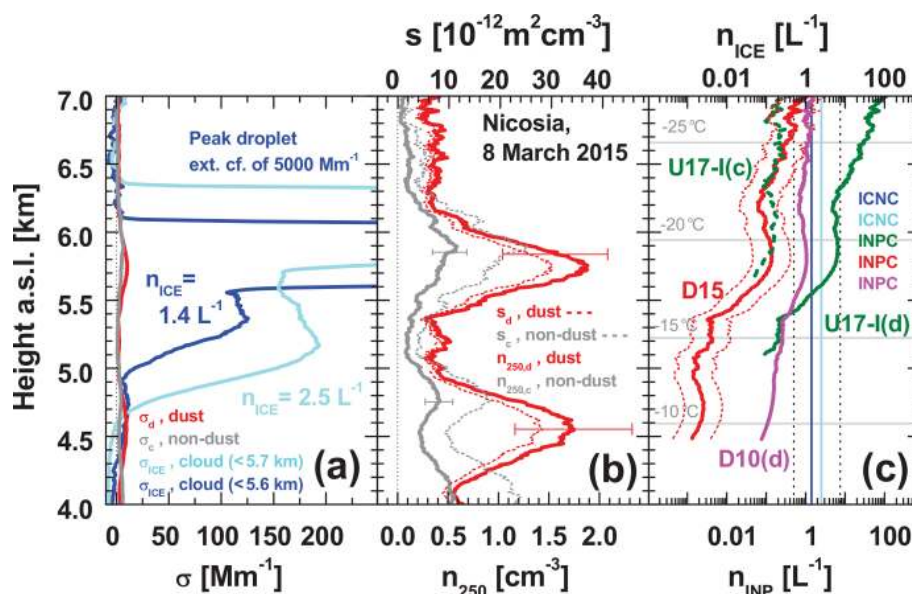
Figure 17. Mixed-phase-cloud INPC–ICNC closure study based on lidar observations over Nicosia on 8 March 2015 (see Fig. 5a and b). (a) Dust (red) and non-dust (grey) particle extinction coefficient (22:00–22:20 UTC mean values, as shown in Fig. 16b), ice crystal extinction coefficient (blue, 22:29–22:31 UTC mean, ice virga from 5 to 5.6 km; light blue, 22:43–22:53 UTC mean, ice virga from 4.7 to 5.7 km), and estimated ICNC values ( n_{\text{ICE}} in blue and light blue for the two time periods); (b) dust (red) and non-dust (grey) particle number concentration n_{250,d} and n_{250,c} (thick lines) and surface area concentration s_d and s_c (thin dashed lines, 22:00–22:20 UTC mean values); (c) INPC values ( n_{\text{INP}} , 22:00–22:20 UTC mean) determined by using the immersion freezing INP parameterizations U17-I(c) (dotted dark green) for non-dust continental aerosol and D10(d) (magenta, thick solid) and D15 (red, thick solid, \text{cf} = 1.0 ), and U17-I(d) (dark green, thick solid) for the dust aerosol fraction. The uncertainty range (factor 3) of each of the four INPC profiles is indicated for D15 only (red dotted lines). The ICNC values (numbers in a) are shown again, but here they are shown as vertical dark-blue and light-blue lines with the overall uncertainty range as vertical black dashed lines.
